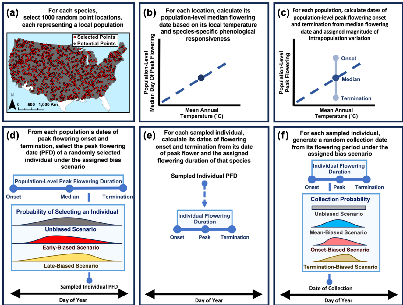
Figure 1. Process by which simulated specimens were generated, beginning by (a) randomly selecting 1000 points for each species, each representing a local population. (b) For each of these points, the median date of peak flowering for a given species was calculated based on the local temperature at that location and the assigned phenological responsiveness of that species. (c) From each population's calculated median date of peak flowering, the dates of peak flowering onset and termination were then calculated using the species' assigned magnitude of intrapopulation variation. (d) From each population's dates of peak flowering onset and termination, we then calculated the duration of peak flowering and randomly selected a date from within that period, which was defined as the date of peak flowering of a single individual selected from that population. While these dates were selected randomly, the probability of selecting each date from within the peak flowering period of a population depended on the type of bias scenario under examination. Individuals could be selected with no bias (shown in grey), with a bias towards collection from the early portion of the population's peak flowering period (shown in red), or with a bias towards collection from the late portion of the population's peak flowering period (shown in yellow). (e) From each individual plant's selected peak flowering date (PFD) we then calculated the dates of that individual's flowering onset and duration (i.e., its individual flowering period) using the individual flowering duration assigned to that species. (f) We then randomly selected a date from within each individual's flowering period to represent the date on which a specimen of that individual was collected. While these dates were selected randomly, the probability of selecting each date from within the peak flowering period of an individual depended on the type of bias scenario under examination. Specimen collection dates were selected either with no bias (shown in grey), with a bias towards collection proximate to the individual's date of peak flowering (shown in blue); with a bias towards collection shortly after flowering onset (shown in red); or with preference towards collection shortly before flowering termination (shown in yellow).
