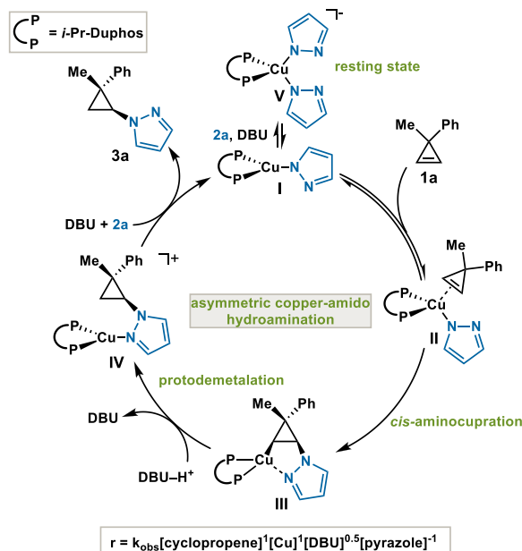
Figure 3. Proposed catalytic cycle.
