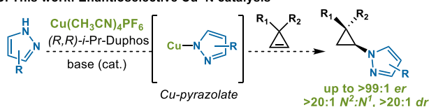
Figure 1. Asymmetric hydroamination of cyclopropenes with pyrazoles.
