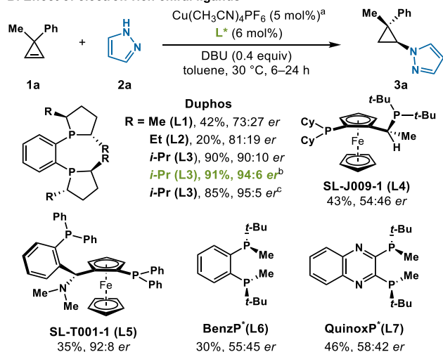
Figure 2. Reaction optimization using bisphosphine ligands. a Reaction conditions: 1a (0.12 mmol), 2 (0.10 mmol), Cu(CH 3 CN) 4 PF 6 (5 mol%), chiral ligand (6 mol%), toluene (0.4 mL), 30 °C, 6–24 h. Yields of isolated products are given. Enantiomeric ratios ( er ) were determined by SFC analysis on a chiral stationary phase. b The reaction was performed using CH 3 CN at 30 °C for 6 h. c The reaction was performed using CH 3 CN at 0 °C for 4 days.
