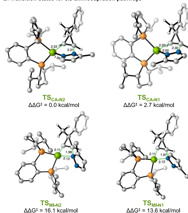
Figure 5. Proposed C–N bond formation pathways and TSs for the favored five-centered 1',6'-migratory insertion of N 2 (TS CA-N2 ) and the higher energy, disfavored four-centered 1,2-migratory insertion of N 2 (TS MI-N2 ).
