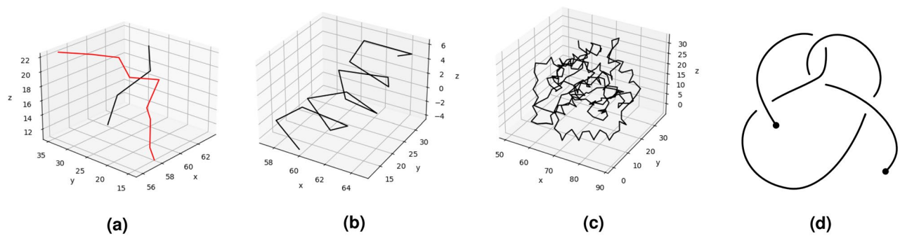
Figure 12. Measures of topological characterization of a knotted protein. The ubiquitin Carboxy-terminal Hydrolase L1 (PDB: 2etl) is used as an example. (a) the black and red curves are parts of the ubiquitin protein, corresponding to residues 26–30 and 215–223, respectively. Their linking number is Lk \approx -0.22 . (b) the writhe and second Vassiliev measure of a helix, residue 192–207, in the ubiquitin protein is Wr \approx 1.65 , while its second Vassiliev measure is v_2 = 0.0 . (c) The second Vassiliev measure of the full length ubiquitin protein, v_2 \approx 1.56 , is indicative of knotting. To be compared to the second Vassiliev measure of the knot 5_2 is v_2 = 2 . (d) An open 5_2 knot.
