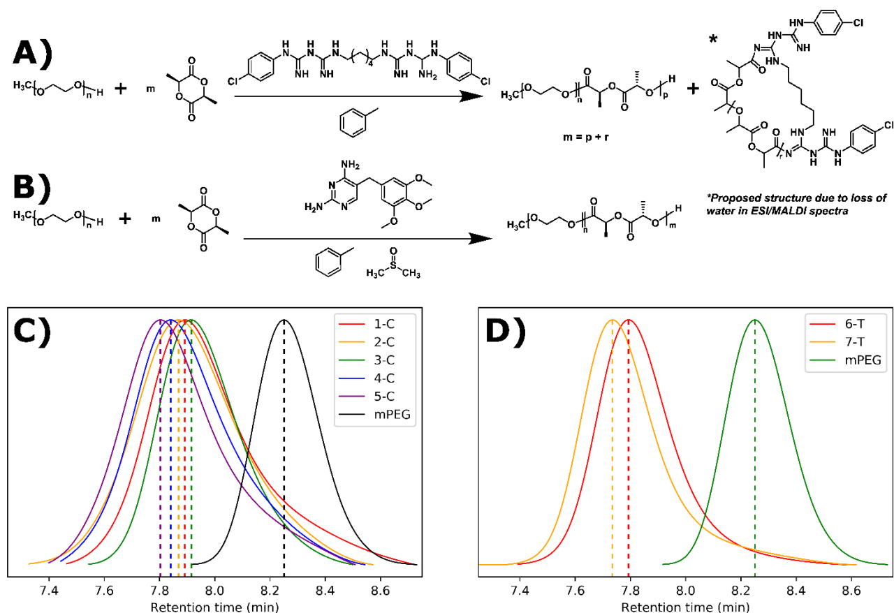
Figure 1: Synthetic scheme and GPC results for guanidine-drug catalyzed ROPI-CDSA: A) chlorhexidine catalyzed and initiated synthesis of PLLA m -b-PEG 45 and PLLA r -chlorhexidine showing a proposed structure for the latter. m , the total equivalents of L-lactide is equal to the equivalents of L-lactide growing off mPEG ( p ) and the equivalents of L-lactide growing off chlorhexidine ( r ). B) trimethoprim catalyzed synthesis of PLLA m -b-PEG 45 . C) and D) GPC data for chlorhexidine and trimethoprim PLLA m -b-PEG 45 series respectively. Note that the retention times of the trimethoprim series is lower than the chlorhexidine series, suggesting the trimethoprim-catalyzed polymer series reaches higher molecular weights than the chlorhexidine-catalyzed series.
