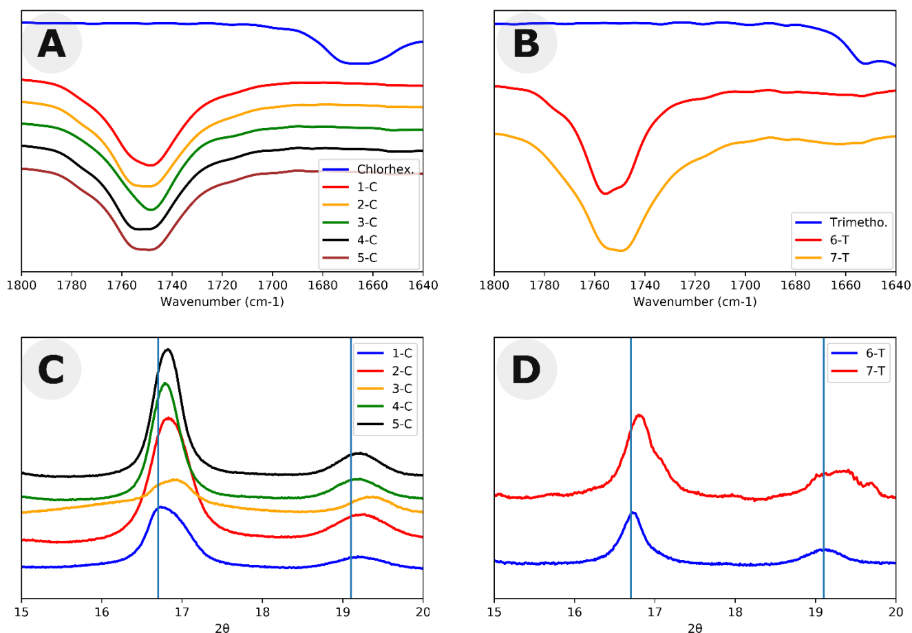
Figure 2: Structural characterization of polymers in this study. FTIR carbonyl spectra for (A) chlorhexidine-catalyzed polymers and (B) trimethoprim-catalyzed polymers. WAXS spectra of the two dominant peaks of (C) chlorhexidine-catalyzed polymers and (D) trimethoprim-catalyzed polymers. Lines represent peaks of 16.7 and 19.1 which are the positions of the two largest WAXS peaks in PLLA.
