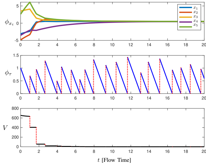
Fig. 3. (top) The x and \tau components of a solution \phi = (\phi_x, \phi_\eta, \phi_\tau) to \mathcal{H} with \mathcal{G} in (37) using Protocol 3.3 which satisfies Theorem 3.8. (bottom) Note that since V_2(\chi) for \mathcal{H} decreases to zero with respect to flow time, it indicates that the solution reaches consensus.
