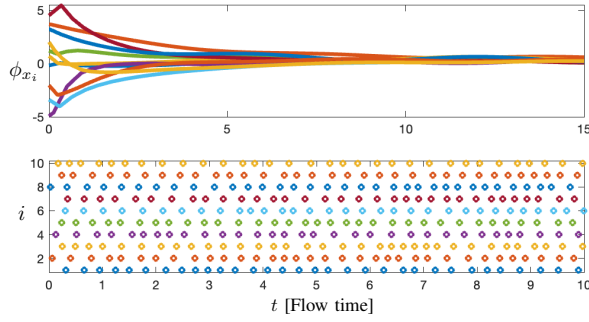
Fig. 6. Robustness of consensus to communication noise for asynchronous communications. The x_i components of a solution \phi = (\phi_x, \phi_\eta, \phi_\tau) to a hybrid system with agent dynamics (2) where asynchronous communication is present. The asynchronous communication is shown on the bottom where an 'o' marker indicates a communication of agent i , more specifically, \phi_{\tau_i}(t, j) = 0 for each (t, j) \in \text{dom } \phi .
