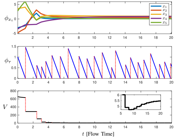
Fig. 7. Input-to-state stability of consensus with communication noise. The x_i and \tau components of a solution \phi = (\phi_x, \phi_\eta, \phi_\tau) to a hybrid system with agent dynamics (2) with synchronous communications. The bottom figure shows the Lyapunov function V in (17) evaluated over the solution.
