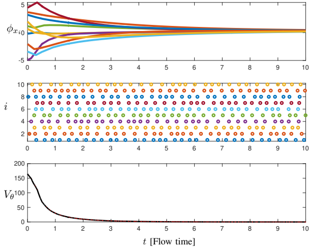
Fig. 4. The x_i components of a solution \phi = (\phi_x, \phi_\eta, \phi_\tau) to a hybrid system with agent dynamics (2) where asynchronous communication is present. The asynchronous communication is shown on the middle chart where an 'o' marker indicates a communication of agent i , more specifically, \phi_{\tau_i}(t, j) = 0 for each (t, j) \in \text{dom } \phi . The Lyapunov function V_\theta in (32) is plotted over time.
