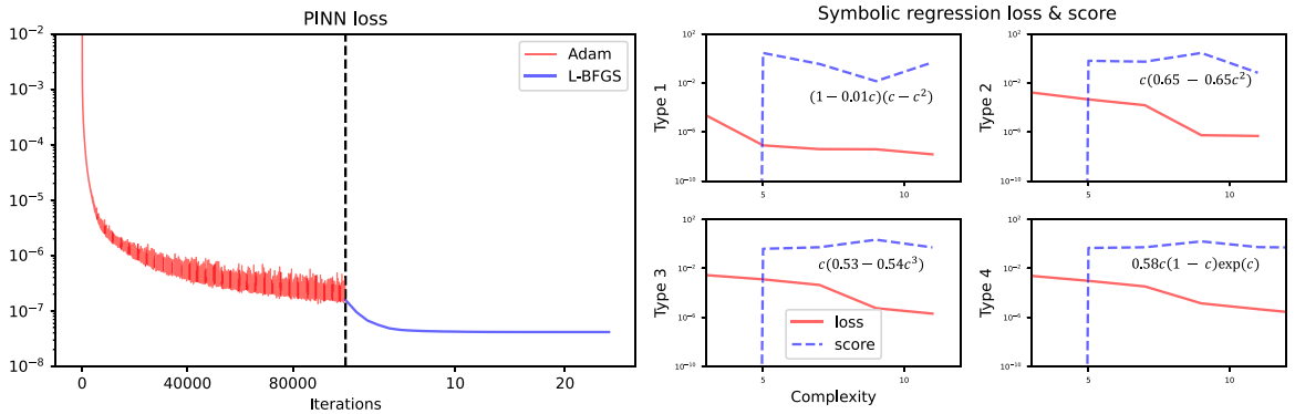
Fig. 3. Losses and evaluation metrics for PINNs and symbolic regression on synthetic data. (Left) Training loss \mathcal{L} = \mathcal{L}_{data} + \mathcal{L}_{res} for PINN. L-BFGS is applied following Adam to ensure convergence. (right) Loss and score for the symbolic regression model at each complexity level. The inferred f_{sym} is highlighted. It aligns with the correct reaction function, and the plateau in loss suggests minimal loss improvement by increasing the expression complexity.
