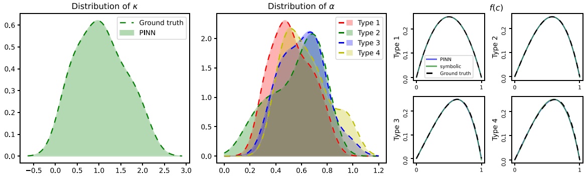
Fig. 2. Parameter and function identification results on synthetic data. Inference results for transport rate (left) and local production rate (middle), as well as the reaction term for each group (right). PINNs accurately identify the distribution of the transport rate at the global level and the distribution of \alpha in each group. The neural network inference result, f_{\phi^*} as well as the symbolic regression approximation, f_{sym} agree with the ground truth f for all four cases.
