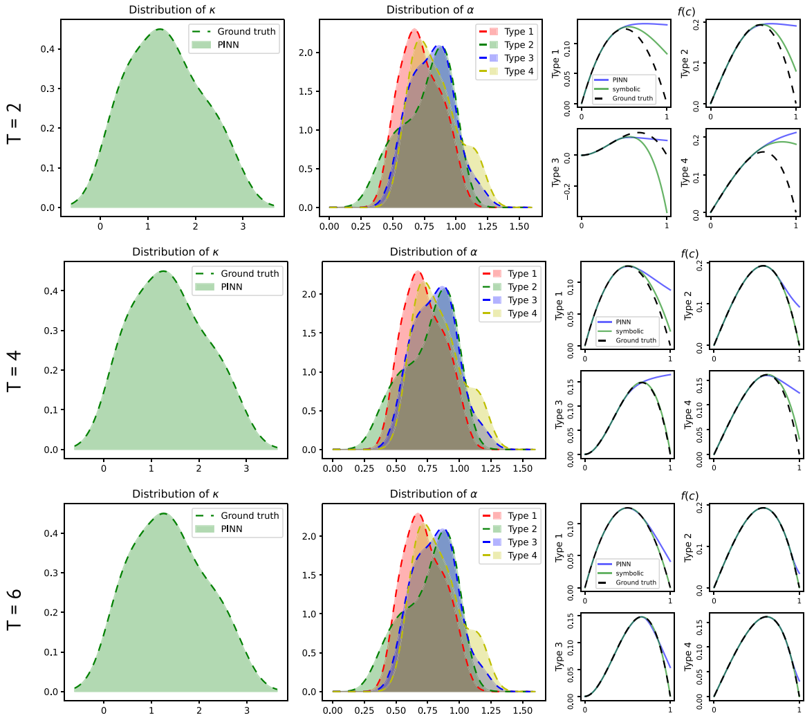
Fig. 7. PINN inference results when T = 2, 4, 6 , without fixed boundary conditions for f . While the learned parameters \kappa and \alpha perform well in all instances, the parametric function f_\phi fails to align with f in regions where there is no available data for c .
