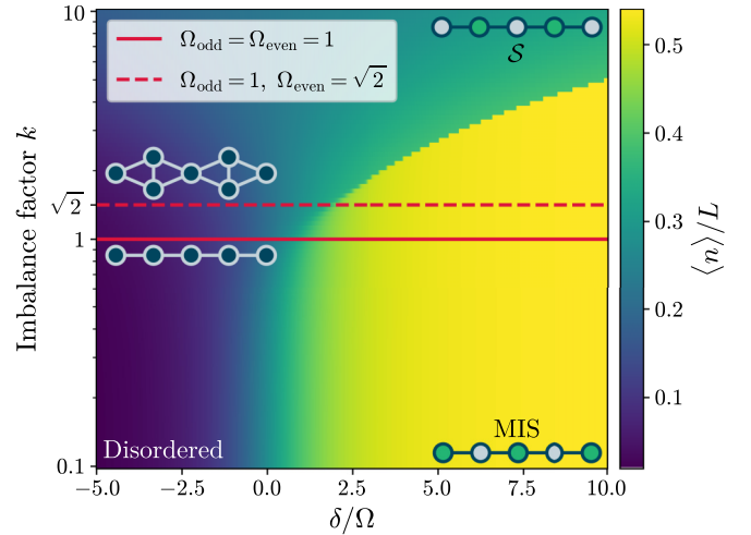
FIG. 3. The mean occupation for a k -PXP chain of length L = 11 with the Rabi frequency enhanced by a factor k on every even site. The doublet chain corresponds to k = \sqrt{2} . The adiabatic sweeps considered originate on the left side for \delta/\Omega \ll -1 and end on the right at \delta/\Omega \gg 1 . The transition from the disordered to the ordered phase along horizontal lines becomes sharper for larger k . Notably, the MIS solution becomes separated by a first-order transition from the phase corresponding to the MIS-1 solution ( S ) when k > 1 . Different k may be realized by other gadgets replacing the doublets (see Appendix B).
