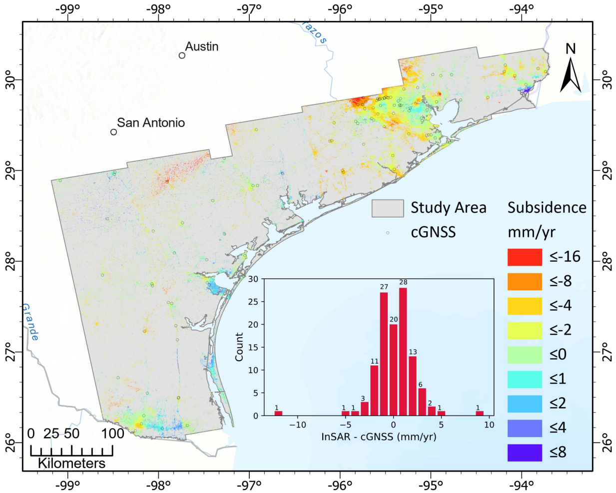
Fig. 5. Land subsidence map represented in 250 m × 250 m grid cells. The lower right subplot visually portrays the distribution of subsidence velocity differences between results obtained using InSAR versus cGNSS, which have been rounded to the nearest whole numbers.
