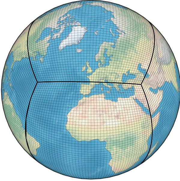
FIG. 1. Depiction of the gnomonic cubed-sphere grid onto which predictors and targets are projected. The cubed sphere is composed of 6 faces with 48^2 = 2304 cells each.
