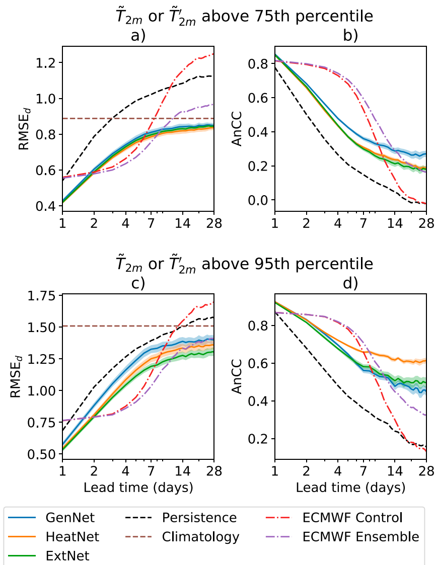
FIG. B1. Forecast metrics for different models during the summer months of 2017–21 and over land. Metrics are shown for forecasts conditioned on either target or forecast standardized temperature anomalies being above the (a),(b) 75th and (c),(d) 95th percentiles of values in the test set. The legend is as in Fig. 3.
