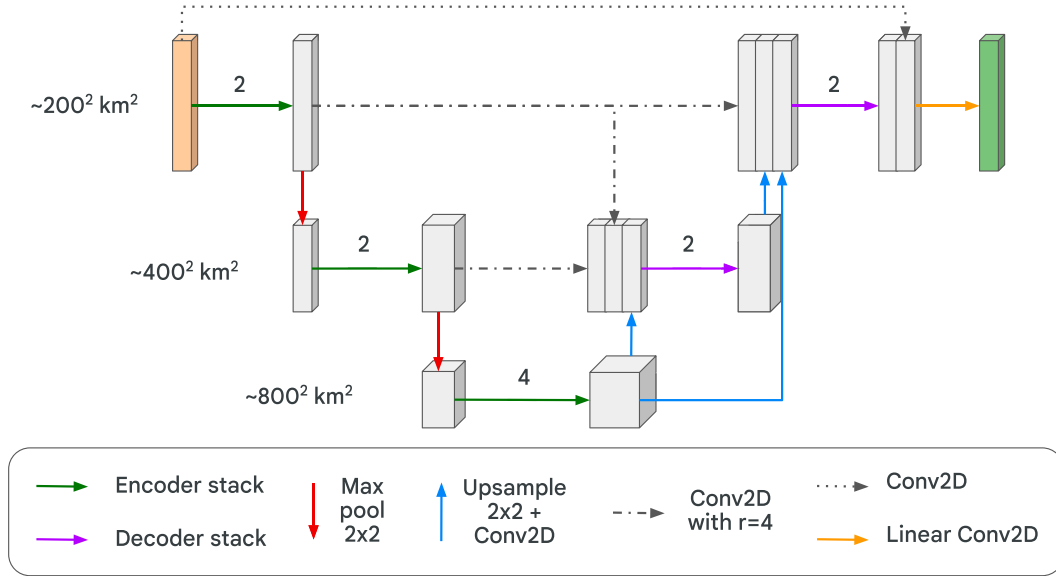
FIG. 2. Neural weather model architecture, modified from a UNet 3+ architecture (Huang et al. 2020). The number of layers of each encoder and decoder stack is as indicated in the schematic. Encoder convolutional layers have geometrically growing dilation factors r = 2^l , where l = 0, 1, \dots is the layer number within the stack from inputs to outputs, and decoder layers have dilation factors r = 8 and 16 . The layers connecting same-level encoders and decoders have convolutions with 32 filters and dilation factor r = 4 . All other layers have dilation factor r = 1 , and all layers have convolutional kernels of size 3 \times 3 . Same-level layers implement 32, 64, and 128 filters in the first, second and third levels, respectively.
