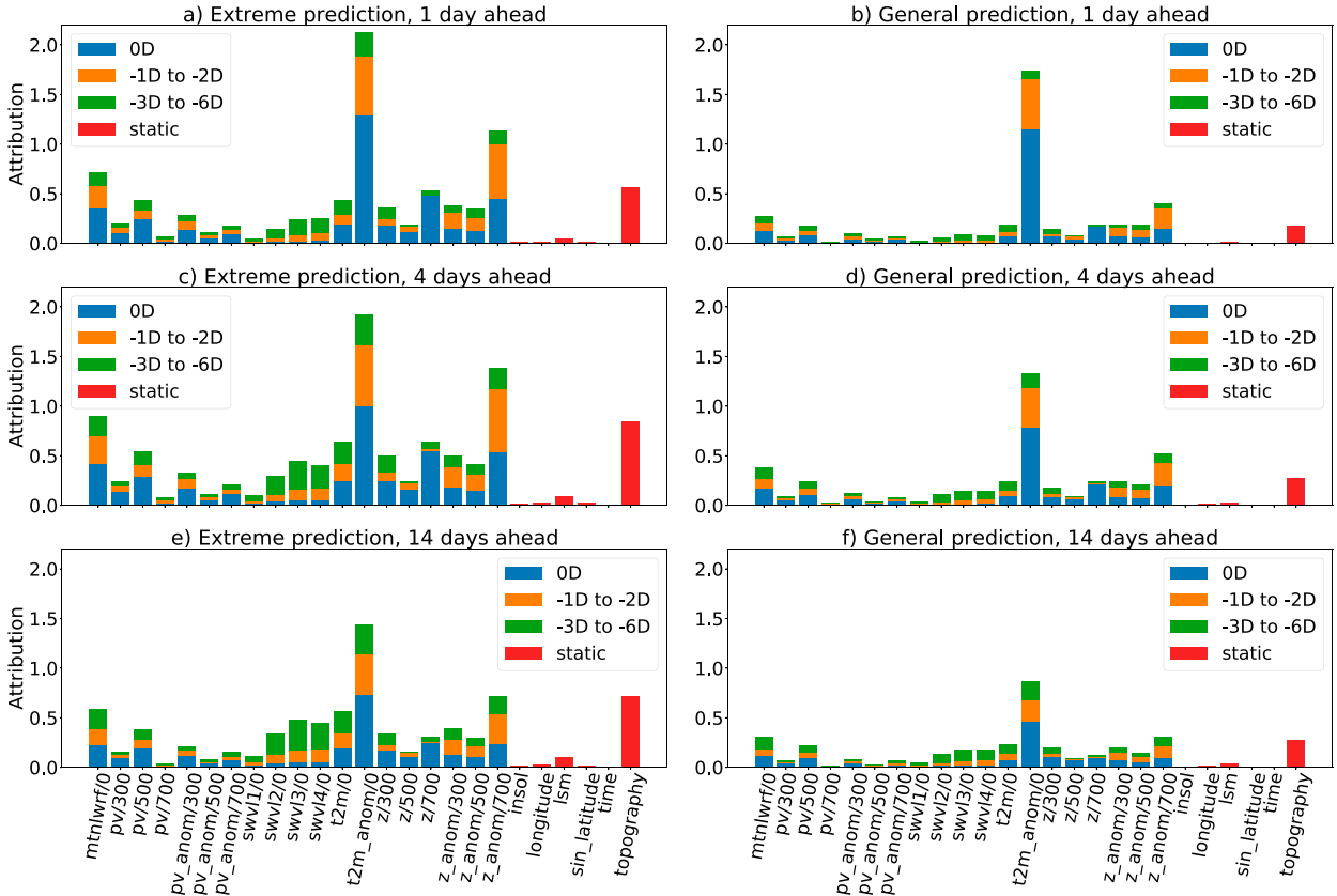
FIG. 8. Forecast feature attribution for summer over land, using data spanning the period 2015–19. Attribution is shown for (a),(c),(e) extreme ( \tilde{T}_{2m} > 2 ) and (b),(d),(f) general prediction, and for different lead times. Feature names follow the notation name/pressure level , where each name follows ECMWF notation: mtnlwr is outgoing longwave radiation, pv is potential vorticity, z is geopotential, swvl is soil water volume at level i below the ground, and t2m is temperature 2 m above the surface. Pressure level 0 represents the land surface. The legend label -iD defines the contribution of data i days before forecast initialization.
