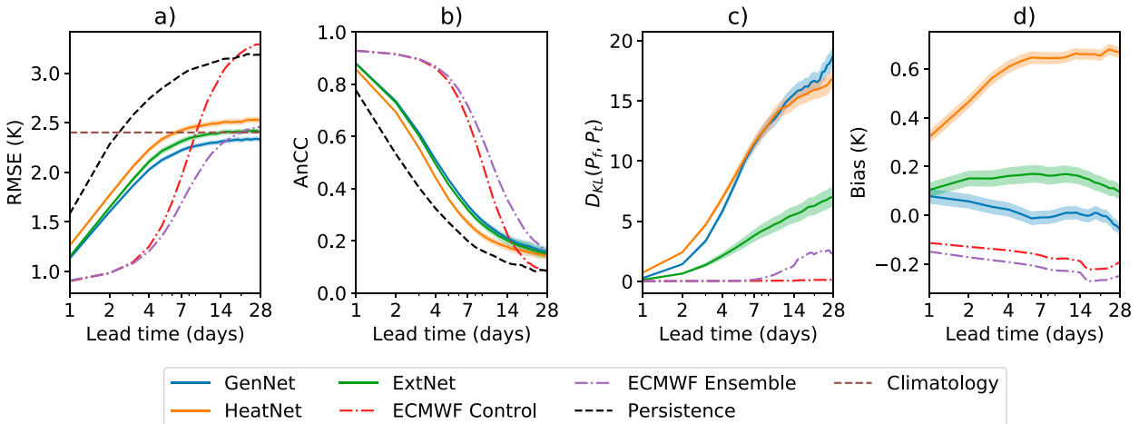
FIG. 5. Forecast metrics for the general 2-m temperature T_{2m} prediction task, for different models as a function of lead time, showing the (a) RMSE, (b) AnCC, (c) Kullback–Leibler divergence D_{KL} of \tilde{T}_{2m} with respect to the targets, and (d) unconditional T_{2m} bias. All results are global and temporal averages over the period 2017–21. NWM names follow section 2b. Uncertainty is defined as in Fig. 3.
