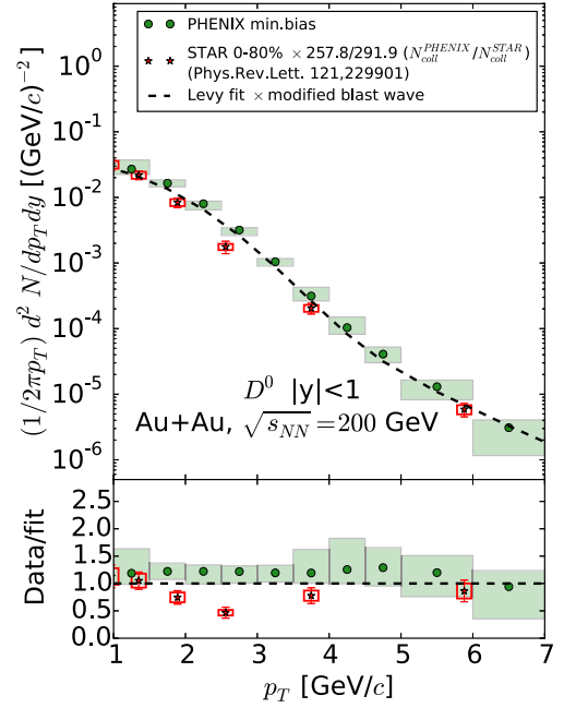
FIG. 12. Unfolded yield of D^0 mesons as a function of p_T at midrapidity |y| < 1 , compared to the measurement from STAR [36].
