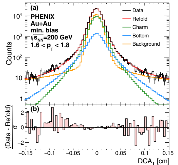
FIG. 8. The measured \text{DCA}_T distribution of (black line) electron tracks, (red line) refolded c + b \rightarrow e , (yellow line) background, (green line) c \rightarrow e , and (blue line) b \rightarrow e in MB Au+Au collisions for 1.6 < p_T < 1.8 GeV/ c .
