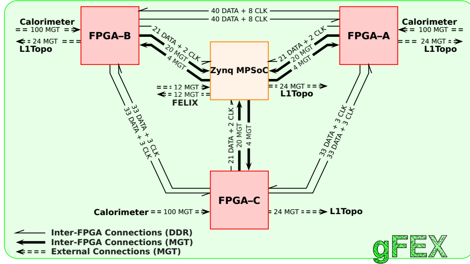
Figure 84. Block diagram of the L1Calo global Feature EXtractor (gFEX).
