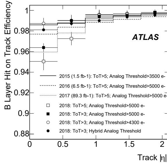
Figure 38. Efficiency for \eta -Layer clusters associated to a reconstructed particle track as a function of the track \eta for different years in Run 2 and different threshold settings at the beginning of 2018. The use of a hybrid setting with lower thresholds for the central modules exposed to higher particle fluence and higher thresholds for forward modules affected by larger occupancy recovers the efficiency obtained in operations at the beginning of Run 2.
