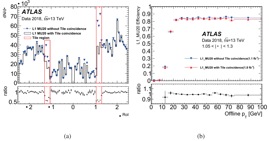
Figure 89. (a) The pseudorapidity distribution of Run 2 L1Muons with p_T > 20 GeV before and after the deployment of the Tile calorimeter coincidence requirement. The reduction in the range 1.05 < |\eta_{\text{RoI}}| < 1.3 , where the coincidence requirement is applied, is highlighted. (b) The efficiency of the Run 2 L1 trigger selection for muon RoIs with p_T > 20 GeV in this pseudorapidity range.
