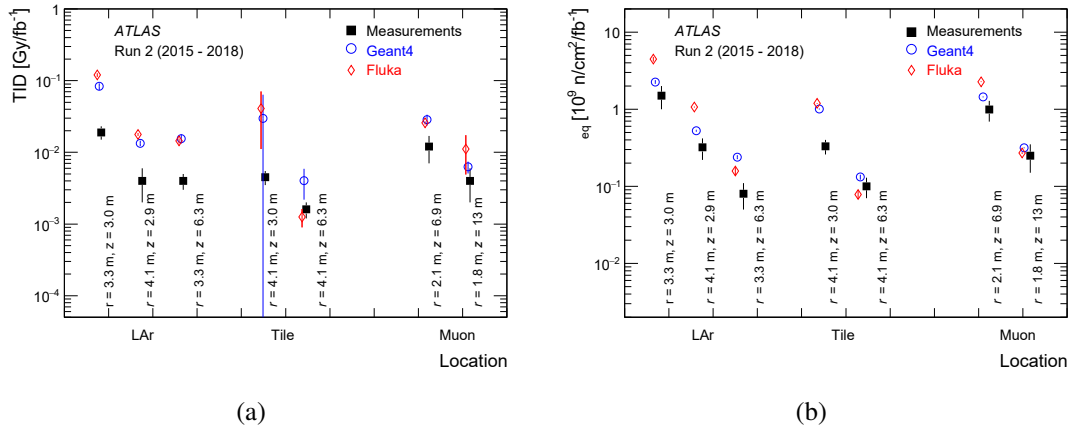
Figure 11. Comparison of measured (a) \text{TID} and (b) \text{Si}_{\text{neq}} in different locations around the calorimeters and the ATLAS muon system. The error bars reflect the statistical uncertainty of the simulations and the variation related to a position uncertainty of the RadMon sensors. Some of the very large error bars for \text{TID} are due to the fact that the quantities are recorded in a small well-shielded volume. Here a single deposition by an energetic electron can dominate and cause a large fluctuation.
