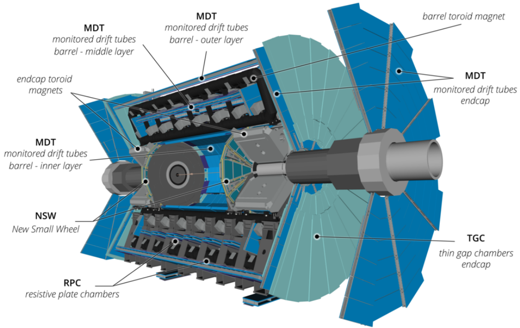
Figure 6. Cut-away view of the ATLAS muon system that detects charged particles exiting the barrel and endcap calorimeters and measures their momentum in the pseudorapidity range 2.7 < |\eta| < 5.0 . The muon system is built around an air-core toroidal magnet system. The main muon detector components upgraded for Run 3 (e.g., the NSWs ) are visible.
