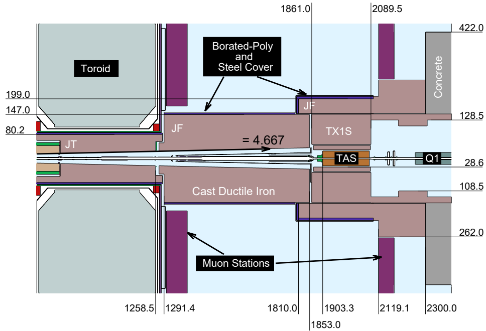
Figure 9. ATLAS forward radiation shielding, as described in the x -symmetric FLUKA geometry. All dimensions are shown in cm. The x dimensions (horizontal axis) are measured from the nominal IP, which is to the left of the left-hand side of the drawing. The y dimensions (vertical axis) are measured from the centre of the beampipe (which is shown in the horizontal centre of the drawing). The role of the TAS absorber is to protect the focusing magnets, e.g. Q1, against particle debris from collisions at the IP. The shielding around the TAS, here labelled “TX1S”, is also referred to as “JN” in some sections of this document. The new JD shielding that supports the NSW of the MS is located to the left of the toroid (outside the region shown in the drawing); the tip of its central hub can be seen projecting into the central opening in the toroid at the far left.
