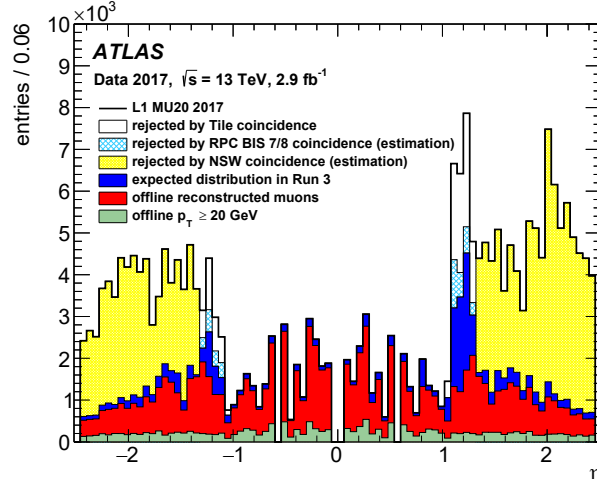
Figure 53. The expected muon trigger rate reduction from the NSW , BIS78 and Level-1 Muon (L1Muon) endcap upgrades; however, the BIS78 on the negative- side, where the fake trigger rate is lower, will only be installed after Run 3.
