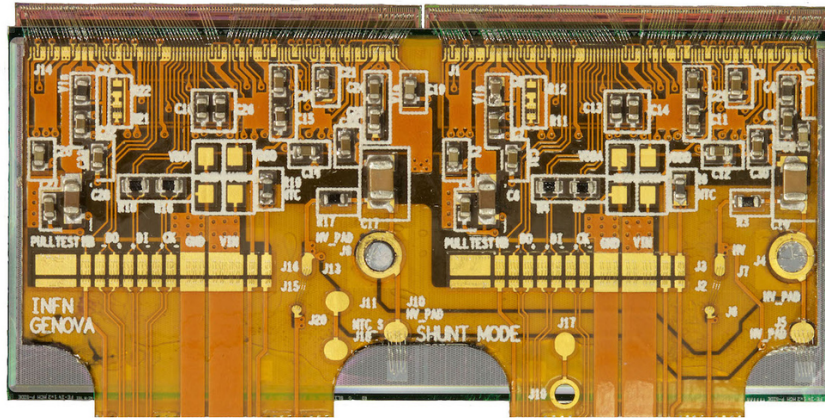
Figure 20. Photograph of an IBL planar module [9]. The full size of the silicon sensor is 18 8 mm 41 3 mm.
