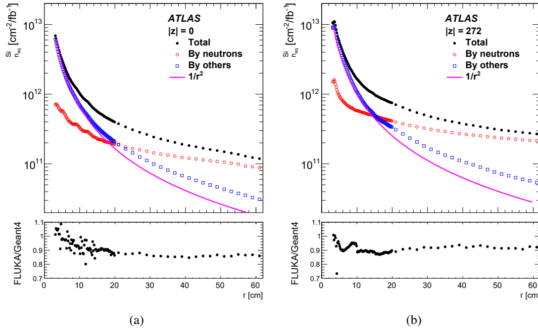
Figure 12. Radial dependence of S_i n_{eq} at (a) |z| = 0 and (b) |z| = 272 cm in the ID, as obtained from FLUKA simulations. The total S_i n_{eq} is divided into the contribution by neutrons and by all other particles. The 1/r^2 dependence is normalised at r = 3 cm to the ‘By others’ value. The lower panels show the ratio of FLUKA and GEANT4 results for the total.
