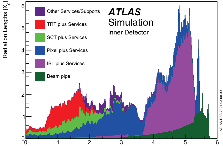
Figure 4. Radiation length ( X_0 ) as a function of |\eta| (averaged over \phi ) for the beampipe and different ID components as implemented in the ATLAS geometry model describing the Run 2 and Run 3 configuration. “Services” refers to supports, cooling infrastructure and cabling.
