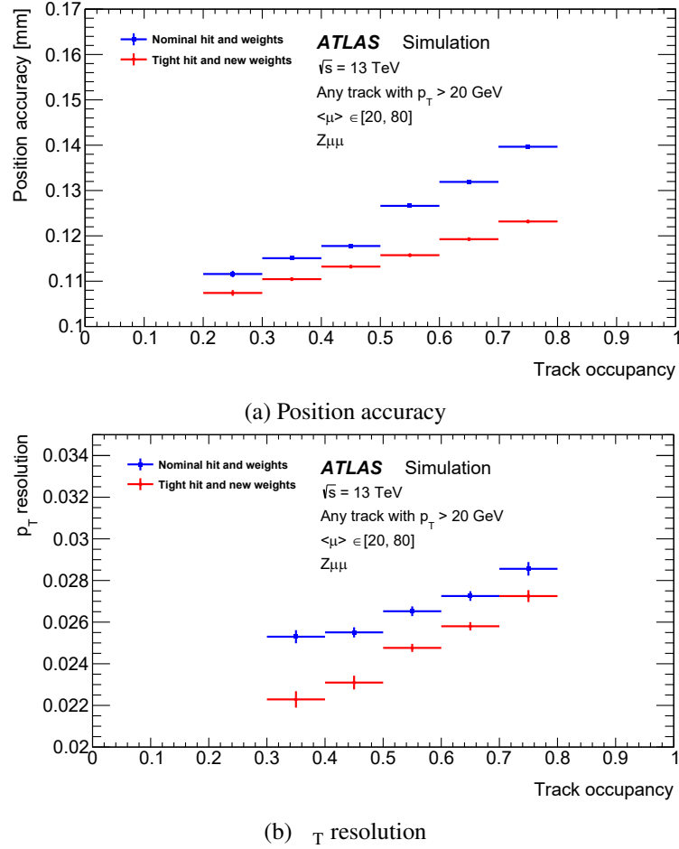
Figure 42. (a) The TRT hit position measurement accuracy and (b) the relative transverse momentum resolution of the ID for tracks with p_T > 20 GeV in simulated events as a function of TRT track occupancy for both the Run 2 hit weights (“nominal”) and the expected Run 3 TRT hit weights (“new”).
