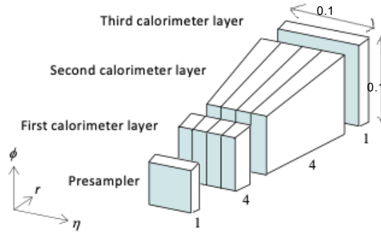
Figure 77. The finer granularity of the Run 3 L1\text{Calo} trigger towers after the upgrade of the liquid argon calorimeter electronics. Each tower is divided into ten Super Cells , each providing an \tau value.
