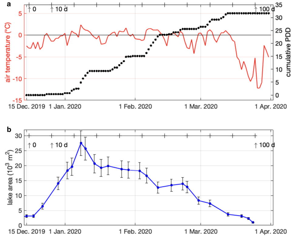
Figure 5. (a) Mean daily air temperature at 2 m above the surface (red line) from the AWS located 40 km northwest of South Doline (see Fig. 1b for ‘AWS’ location), and cumulative positive-degree days (PDD; black dots) calculated from these same air temperature data. (b) Area of surface ponding in the doline basin through the 2019/2020 melt season (blue dots/line with black error bars), calculated from orthorectified time-lapse photos. As a point of reference, we estimate the total area of the doline basin floor to be \sim 6 \times 10^4 \text{ m}^2 .
