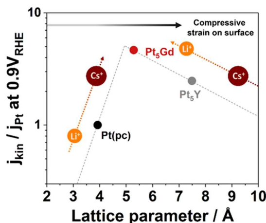
Figure 5. Relative ORR activity at 0.9 V vs RHE as a function of lattice parameter in \text{O}_2 -saturated 0.1 M \text{HClO}_4 for Pt(pc), \text{Pt}_5\text{Gd} , and \text{Pt}_5\text{Y} electrodes (corresponding to black, red, and gray circles, respectively) and their ORR activity-trend measured in 0.1 M \text{O}_2 -saturated alkaline solutions with dashed arrows. The induced strain (compression) on the surface increases with a larger lattice parameter. It is noted that the dashed lines of the pseudo volcano plot only represent the guides to the eyes, and the lattice parameters of measured electrodes are referred to the experimental XRD patterns in the Supporting Information in agreement with refs 10, 32, and 35.
