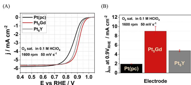
Figure 2. (A) i R-corrected voltammograms with anodic scan and (B) bar chart of the j_{\text{kin}} at 0.9 V vs RHE of the Pt(pc), Pt 5 Gd, and Pt 5 Y electrodes in O 2 -saturated 0.1 M HClO 4 with the scan rate of 50 mV s -1 at 1600 rpm.
