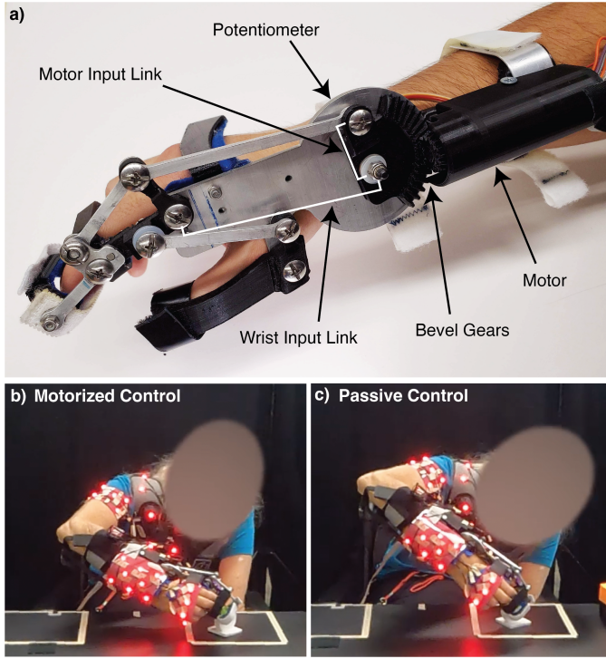
Fig. 1. a) Motorized Wrist-Driven Orthosis (MWDO), from [28]. When using motorized control, the potentiometer measures wrist angle via wrist input link position and the motor correspondingly drives the bevel gears to rotate the position of the motor input link. b) A participant with SCI operating the MWDO with motorized control. c) The participant operating the MWDO with passive control (motor off).
