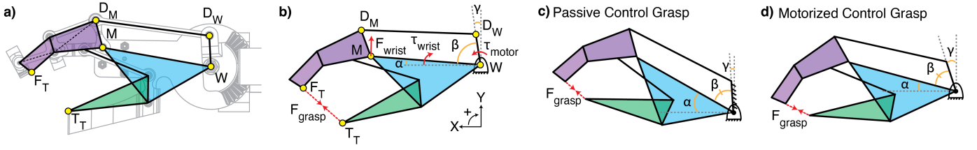
Fig. 2. a) Schematic of MWDO mechanism. Shaded regions represent rigid bodies for analysis. b) Force and torques for MWDO actuation. Variables are defined in the main text. c) Example of grasping in the passive control state, requiring a larger wrist extension angle, \alpha , when compared to d) grasping in the motorized control state to achieve the same grasp aperture. \beta remains constant regardless of control state when grasping objects of the same size.
