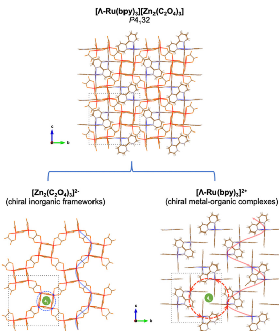
Fig. 1 Crystal structure of [\Lambda\text{-Ru}(\text{bpy})_3][\text{Zn}_2(\text{C}_2\text{O}_4)_3] (top): a 3-connected (10,3) oxalate-based anionic framework, [\text{Zn}_2(\text{C}_2\text{O}_4)_3]^{2-} (bottom left), and the embedded cationic metal complexes, [\text{Ru}(\text{bpy})_3]^{2+} (bottom right).
