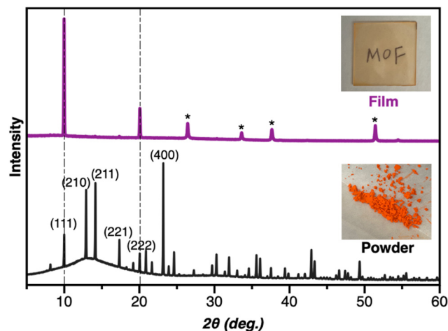
Fig. 2 PXRD of [\text{Ru}(\text{bpy})_3][\text{Zn}_2(\text{C}_2\text{O}_4)_3] . Top: [\text{Ru}(\text{bpy})_3][\text{Zn}_2(\text{C}_2\text{O}_4)_3] thin film on FTO glass (asterisk label the peaks from FTO glass substrate); bottom: [\text{Ru}(\text{bpy})_3][\text{Zn}_2(\text{C}_2\text{O}_4)_3] powder.
