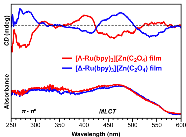
Fig. 3 UV-Vis absorption spectra and CD spectra of the [\Lambda/\Delta\text{-Ru}(\text{bpy})_3][\text{Zn}_2(\text{C}_2\text{O}_4)_3] film on a glass substrate.
