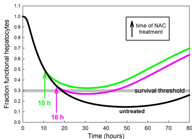
Figure 5. Rescue by N-acetyl Cysteine. The black curve shows the response of the male to an 18-gm dose of APAP if not treated. The result is almost certain liver failure. The green curve shows the NAC rescue of the male by the protocol described in the text starting 10 h after ingestion. The pink curve shows rescue by NAC starting at 16 h after ingestion; rescue is possible but problematic.
