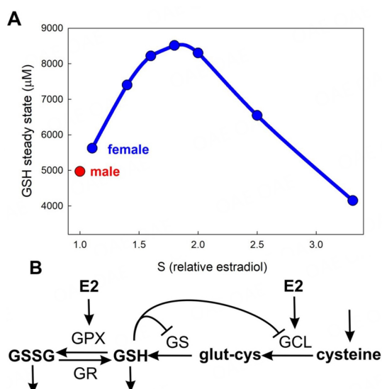
Figure 2. Consequences of the GSH regulatory motif. Panel B shows the GSH regulatory motif (taken from Figure 1), including the effects of estradiol and the inhibition of GCL and glutathione synthetase (GS) by GSH. Panel A shows the steady state value of GSH as a function of the parameter S , which increases with estradiol concentration and is defined in formula (2). The GSH curve goes up for low estradiol values, reaches a peak and descends for high estradiol values. The reasons for this behavior are discussed in the text.
