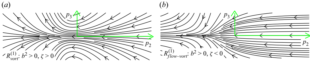
Figure 5. Phase portraits of (5.2) and (5.10) in the b^2 > 0 regime in the gradient ( p_2 )–vorticity ( p_3 ) plane with \zeta > 0 (a) and \zeta < 0 (b). When b^2 > 0 and \zeta > 0 , i.e. in (a) representing R_{vort}^{(1)} close to the flow gradient plane ( p_3 = 0 ), the p_3 component of the phase velocity changes sign from negative to positive along with an increase in magnitude downstream of the p_2 = 0 plane indicating a departure of a particle from the flow gradient plane at a rate higher than it approaches the plane. However, when b^2 > 0 and \zeta < 0 , i.e. in (b) representing R_{flow-vort}^{(1)} the p_3 component of the phase velocity is negative for all p_2 indicating an approach towards the flow gradient plane. Since p_2 never approaches zero on the flow gradient plane for b^2 > 0 it is an unstable and stable limit cycle for R_{vort}^{(1)} ( \zeta > 0 , a) and R_{flow-vort}^{(1)} ( \zeta < 0 , b), respectively.
