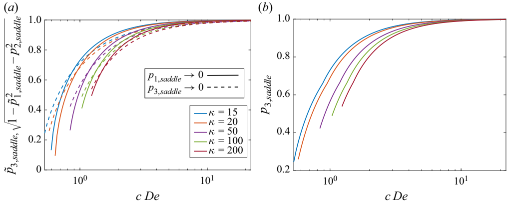
Figure 14. The p_3 coordinate of the saddle point in the flow–vorticity plane in R_{\text{flow-vort}}^{(2)} and R_{\text{flow-vort}}^{(3)} .
