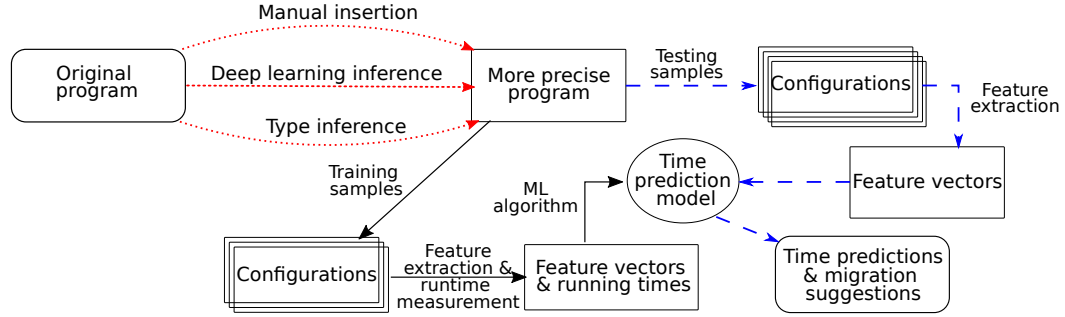
■ Figure 2 Workflow of LearnPerf . Solid arrows denote information flow in training phase and dashed, blue arrows denote that in prediction phase. Dotted, red arrows denote type annotation additions, and they are not a part of this work.
