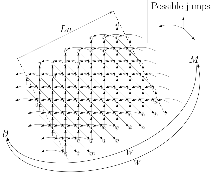
Figure 2: Graph \mathcal{H}_{N,L} . Here \mathcal{N} = \{(0,1), (1,-1), (-2,0)\} , and v = (2,1) . Boundary conditions in direction perpendicular to v are periodic; vertices labeled with the same letters are identified. Arrows to and from the main part of the graph on the left are understood to originate from or terminate at \partial , and similarly with M on the right side.
