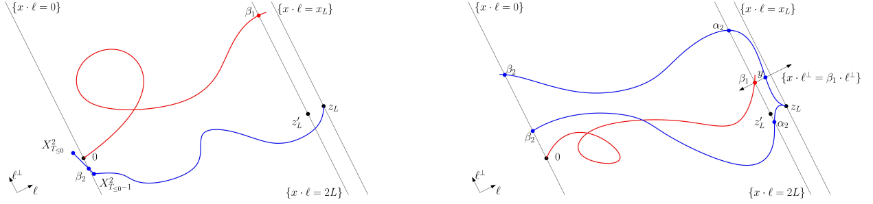
Figure 1: On the left, we have (X_{T_{\geq 2L}}^1 - z_L) \cdot \ell^\perp > 0 and X_{T_{\leq 0}}^2 \cdot \ell^\perp > 0 , but \beta_2 \cdot \ell^\perp < 0 . On the right, different ways to have \beta_2 \cdot \ell^\perp, (\beta_1 - z'_L) \cdot \ell^\perp > 0 are depicted. The upper path from z_L shows the situation \alpha_2 \cdot \ell^\perp > \beta_1 \cdot \ell^\perp , while the lower path from z_L shows \alpha_2 \cdot \ell^\perp < \beta_1 \cdot \ell^\perp .
