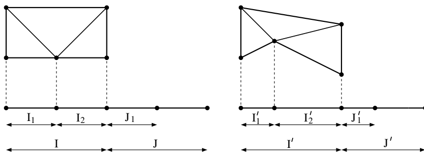
Figure 4. Here I' = \varphi(I) , and similarly for the other intervals. If K = I \cup J is a dyadic interval, then \mu can be bounded directly in terms of \text{qs}(\varphi, I) , \text{qs}(\varphi, J) , \text{qs}(\varphi(I \cup J)) . In general, I \cup J is not in the same dyadic family as I and J , so we have to estimate the last term using a sum over the multi-resolution family obtained by the “ \frac{1}{3} -trick”.
