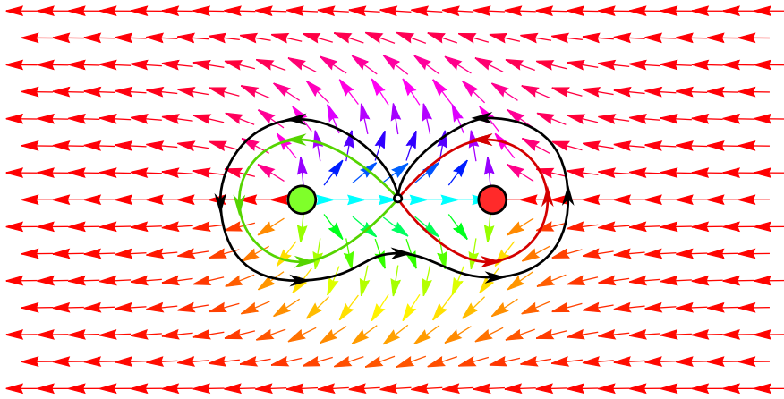
Fig. 21. Defect and anti-defect pair in 2D. Two monopoles of charge +1 (green dot) and −1 (red dot) respectively, are detected by computing the winding number along the green and red path. The black path that encircles both gives rise to a total topological charge Q = 0 , demonstrating additivity.
