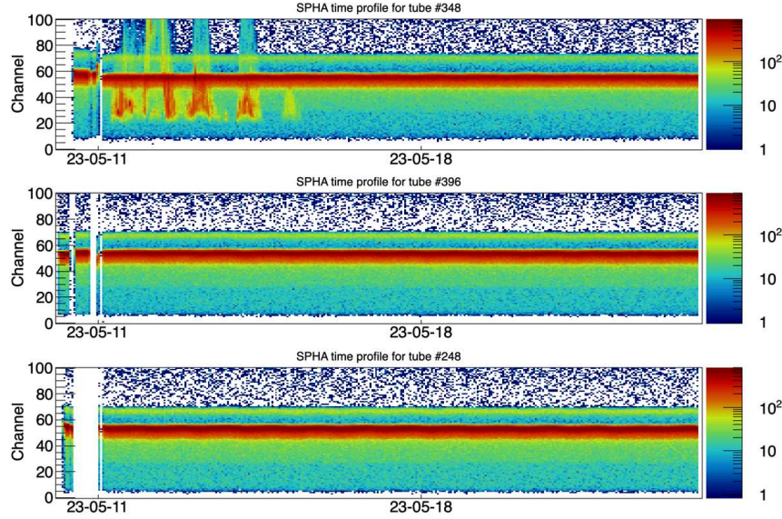
Figure 8: BP-28 tube counts over time. Long-term tests for 3 tubes. Top: tube 348. Middle: tube 396. Bottom: tube 248
