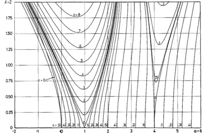
FIG. 9. Arnold tongues of the damped Mathieu equation. The x axis is the drive frequency expressed via the dimensionless ratio a = (2\omega_0)^2/\omega_D^2 , while the y axis is the drive amplitude \delta . Contours indicate the critical drive amplitude required for resonance when the coefficient of friction takes a given value c . When c > 0 , the period-doubled solution onsets only at finite \delta . Adapted from Pedersen, 1980.
