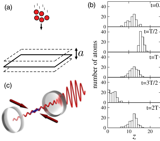
FIG. 8. (a) Schematic depicting N atoms bouncing off an oscillating mirror (Sacha, 2015). (b) Numerical simulations of the scenario in (a) shows that the time evolution of the atomic density exhibits SzB. At each time shown, the positions of 10^2 atoms (out of 10^4 ) are measured and a histogram of those positions is depicted. (c) A Bose-Einstein condensate in a transversely pumped high-finesse optical cavity can realize signatures of SzB in an open system. In particular, the atom-cavity system can exhibit a period-doubled oscillation between distinct density wave patterns (Keßler et al., 2021). (a)–(c) Adapted from Sacha, 2015, Sacha and Zakrzewski, 2018, and Keßler et al., 2021.
