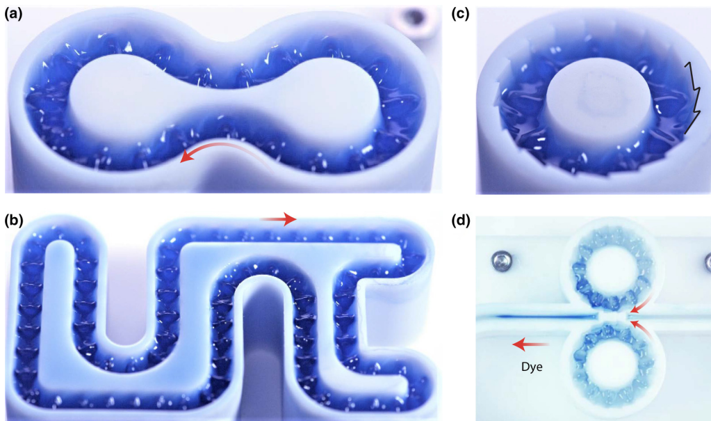
FIG. 2. Traveling Faraday waves in complex geometries. Traveling Faraday waves may also move along (a) channels with variable curvature, and (b) more complicated networks including both straight and curved sections. (c) The direction of motion can be fixed by including ratchets on the channel's vertical walls. (d) Small-scale fluid pumps may be created by connecting channels with ratcheted walls to a secondary fluid channel. Drops of blue dye have been added in (d) to demonstrate the fluid's unidirectional transport.
