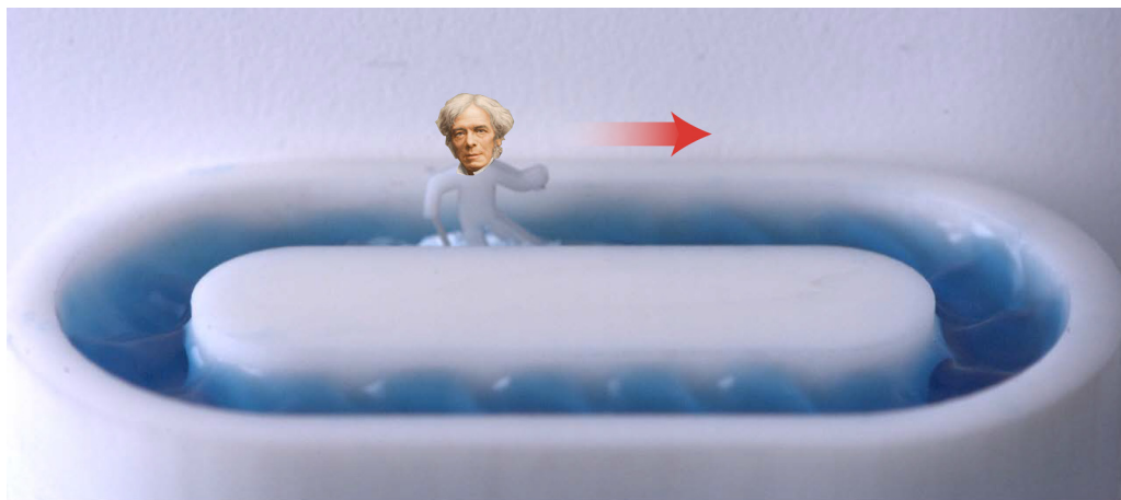
FIG. 3. Transport of floating objects. A 3D-printed figurine suspended on the liquid-gas interface is transported along the channel by traveling Faraday waves, illustrating the potential of this instability as a new mechanism for the transport of granular materials floating on interfaces. The speed of the object is proportional to the wave speed. An image of Michael Faraday was digitally added in reference to the title of the video, “Run, Faraday, run,” and the playful reference to the famous line “Run, Forrest, run” from the movie Forrest Gump .
