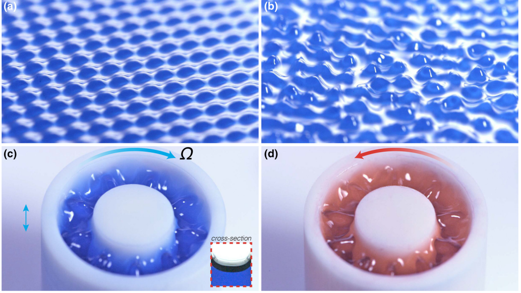
FIG. 1. Symmetry-breaking of Faraday waves. (a) Standing surface waves emerging when a liquid layer is vibrated vertically at a driving acceleration just above the so-called Faraday threshold. (b) The uniform Faraday pattern becomes chaotic as the driving acceleration is increased further due to a secondary order-disorder instability. (c), (d) Faraday waves in an annular channel start to rotate at rate \Omega when the channel width W , the Faraday wavelength \lambda , and the capillary length l_c are all comparable. The symmetry is spontaneously broken; the direction of motion, (c) clockwise or (d) counterclockwise, is random, but persistent once one direction is selected.
