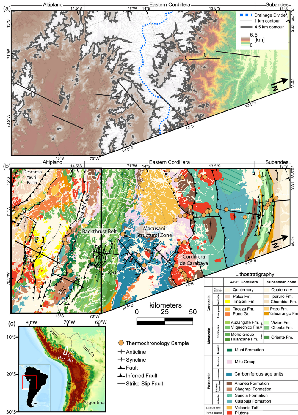
Fig. 1. (a) Topographic map (based on ASTER GDEM) of the study area with bolded 4500 m contour and drainage divide between systems that drain northward and southward, I=interfluvial, C=canyon. (b) Geologic map (modified from Sánchez and Zapata (2003), Cerrón and Chacaltana (2003), Monge Miguel and Montoya Pérez (2003) and Perez et al. (2016b) with published thermochronology sample locations (Clark et al., 1990; Falkowski et al., 2023; Farrar et al., 1988; Kontak et al., 1987, 1990a; Lease and Ehlers, 2013; Perez, 2015; Perez et al., 2016b) (inset box corresponds to Fig. 4). Black lines in (a) and (b) represent balanced cross-section lines. The lines are proximal to field observations and oriented normal to the structural trend, which changes from ~N 20° E to N 60° E in the Macusani Structural Zone (Perez et al., 2016a), resulting in multiple breaks in the section. Breaks are positioned at major structures (Perez et al., 2016b). (c) Digital topography of the Central Andes, WC is Western Cordillera, AP is Altiplano, EC is Eastern Cordillera, SA is Subandean Zone. White box marks location of (a) and (b).
