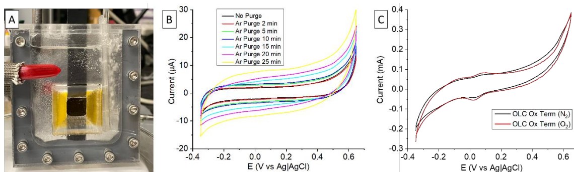
Figure 4 (A) PMMA electrochemical cell with carbon paper working electrode while purging with argon on the right. (B) Cyclic voltammetry of carbon paper before and after argon purging at different times. (C) Cyclic voltammetry of carbon paper after nitrogen and oxygen purging.
