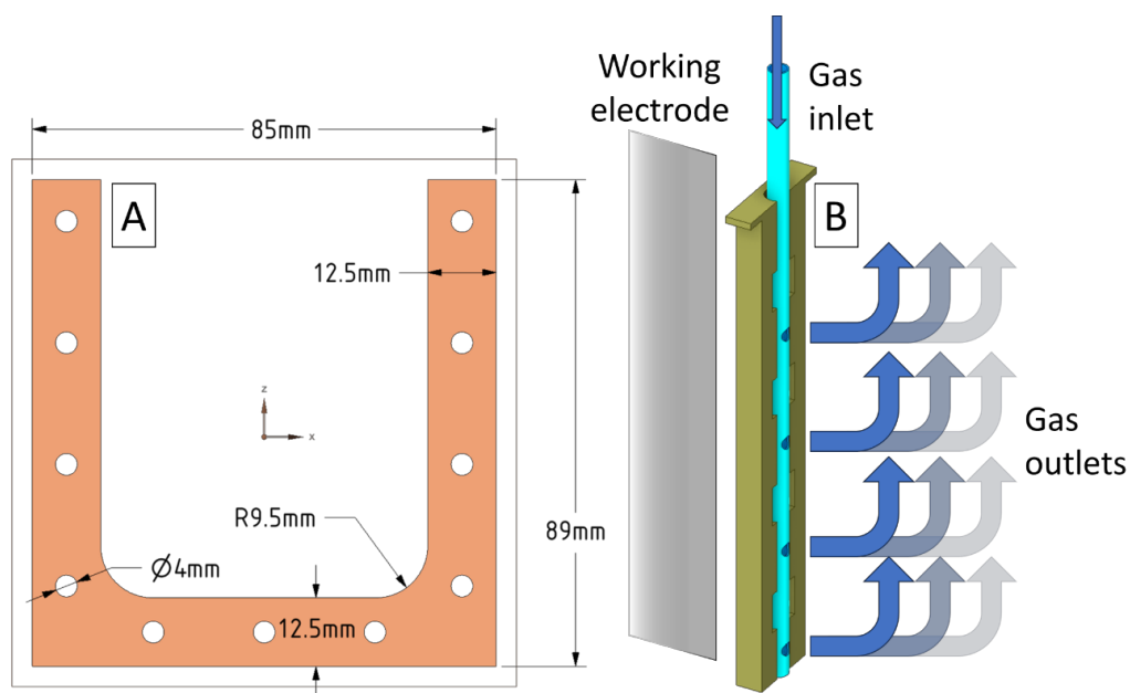
Figure 2 (A) Gasket size for the electrochemical cell used and (B) diagram of gas purging to the side contrary to the working electrode to avoid bubbles that would affect XAS measurements.
