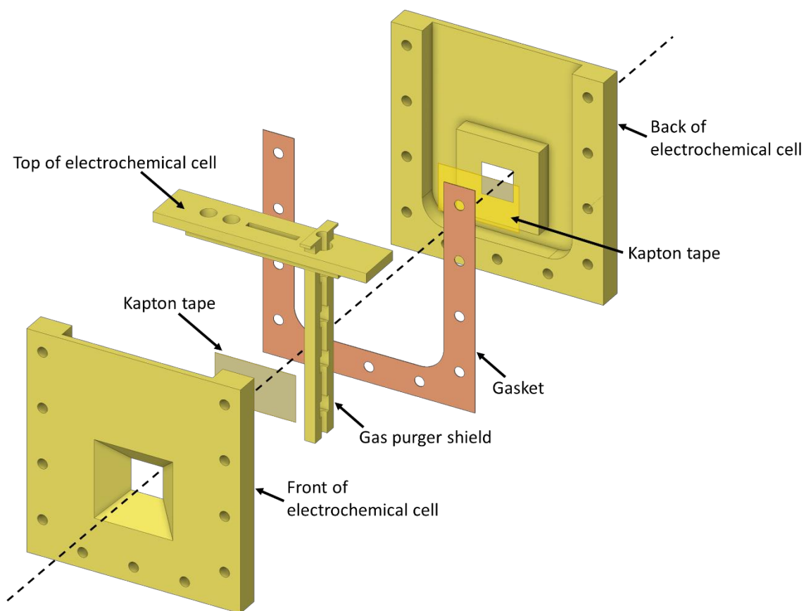
Figure 1 Exploded view of the electrochemical cell.
