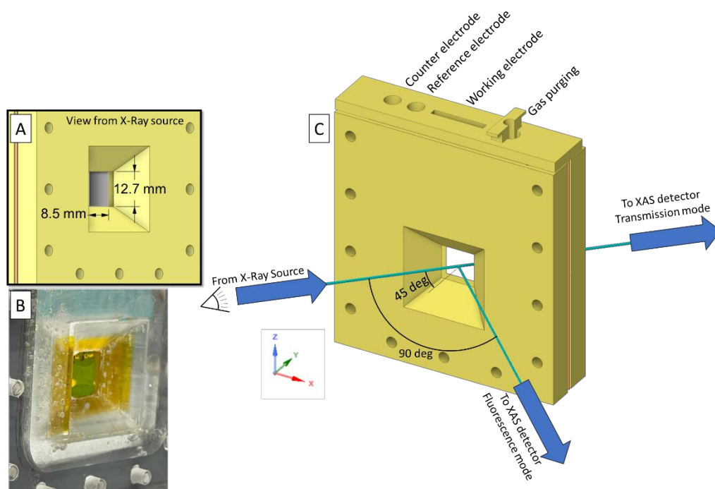
Figure 3 (A) X-Y in plane 45° view to Y axis (view from X-ray source) of the sample using a 254 \mu\text{m} gasket with a sample window of 8.5 mm by 12.7 mm for XAS experiments. (B) Same view in the PMMA electrochemical cell used for in situ XAS experiments. (C) Diagram of the electrochemical cell with position of electrodes, gas purging, and relative positions for the X-ray source and XAS detectors in transmission and fluorescence modes.
