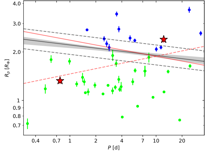
Fig. 6. R_p vs P distribution representing the planets in our Msample . Planets classified above and below the radius valley are shown in blue and green, respectively, while the red star-shaped markers are for TOI-732 b and c. The radius valley inferred via the SVM-based method is marked by the solid grey line with the shaded region highlighting the 1\sigma limits of the best-fit line. The two parallel dashed grey lines are the median boundaries passing through the supporting vectors that determine the location of the solid line. Finally, the red lines represent the theoretically expected R_{p,\text{valley}} boundary in case of a thermally-driven mass-loss scenario (solid line as computed from Affolter et al. 2023; negative slope) and the R_p upper limit of planets borned rocky in a gas-empty disc (dashed line as computed from Lopez & Rice 2018; positive slope).
