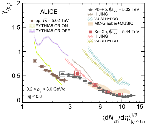
Fig. 3. Standardized skewness \gamma_{(p_T)} shown as a function of \langle dN_{ch}/d\eta \rangle_{|\eta|<0.5}^{1/3} in Pb–Pb collisions at \sqrt{s_{NN}} = 5.02 TeV, Xe–Xe collisions at \sqrt{s_{NN}} = 5.44 TeV, and pp collisions at \sqrt{s} = 5.02 TeV. The predictions from different event generators and hydrodynamic model calculations from V-USPHYDRO [17] and MC-Glauber+MUSIC [40,41] are denoted by colored bands. The statistical (systematic) uncertainties are represented by vertical bars (boxes).
