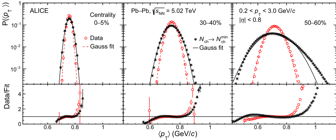
Fig. 2. Comparison of event-by-event mean transverse momentum \langle p_T \rangle distribution from actual analysis and modified analysis in which N_{ch} in each event is fixed to N_{ch}^{min} ( N_{ch}^{min} is the minimum number of charged particles in a given centrality class) and N_{ch}^{min} number of particles are selected in each event randomly for the 0–5% (left), 30–40% (middle), and 50–60% (right) centrality classes.
