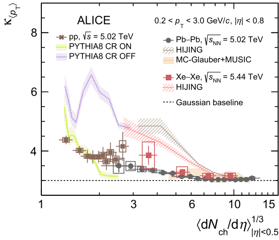
Fig. 5. Kurtosis \kappa(p_T) shown as a function of (dN_{ch}/d\eta)_{|\eta|<0.5}^{1/3} in Pb-Pb collisions at \sqrt{s_{NN}} = 5.02 TeV, Xe-Xe collisions at \sqrt{s_{NN}} = 5.44 TeV and pp collisions at \sqrt{s} = 5.02 TeV. The predictions from different event generators and hydrodynamic calculations from MC-Glauber+MUSIC model [40,41] are represented by colored bands. The dashed line indicates the Gaussian baseline. The statistical (systematic) uncertainties are represented by vertical bars (boxes).
