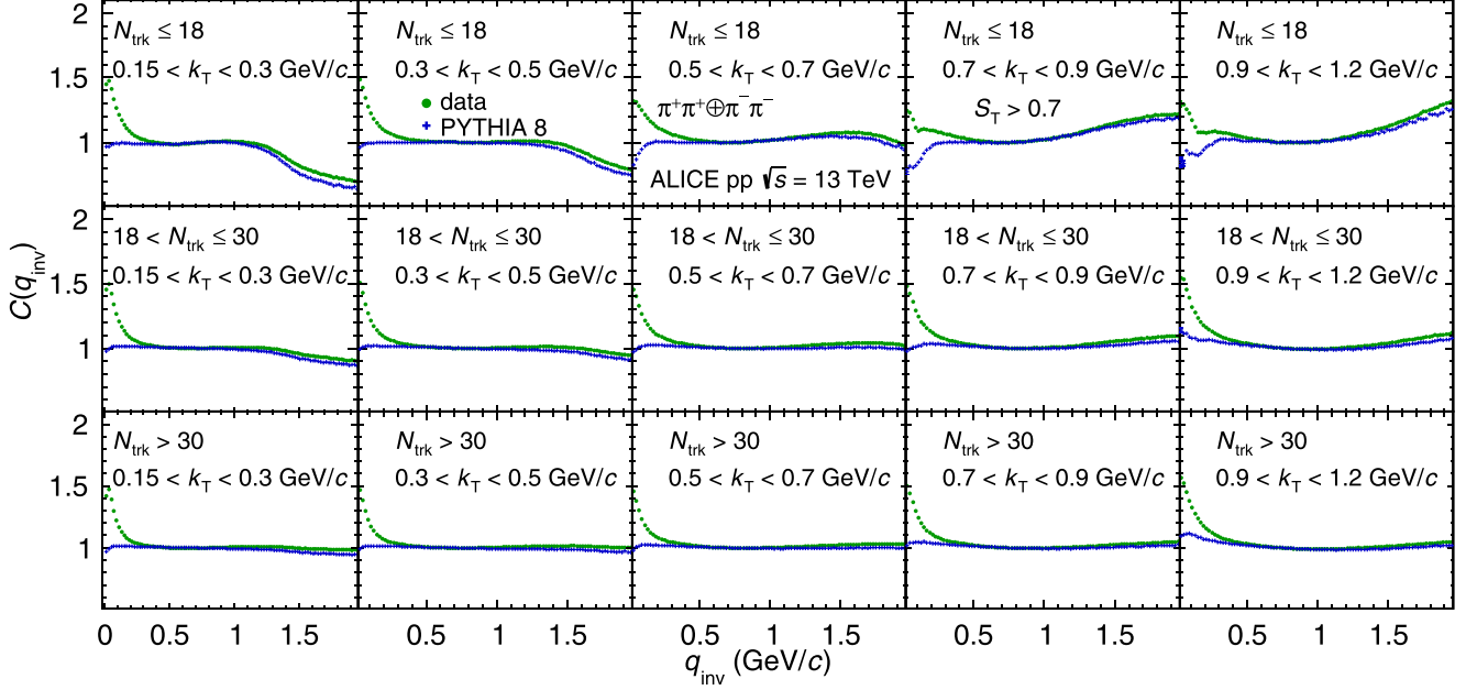
FIG. 3. The \pi^\pm\pi^\pm experimental correlation functions (green solid circles) as function of the invariant pair relative momentum q_{\text{inv}} in pp collisions at \sqrt{s} = 13 TeV for the raw multiplicity N_{\text{trk}} intervals of (1–18), (19–30), and ( >30 ) in the (0.15–0.3), (0.3–0.5), (0.5–0.7), (0.7–0.9), and (0.9–1.2) GeV/ c k_T intervals. A sphericity selection of S_T > 0.7 is applied. The data are compared with PYTHIA 8 calculations, shown by blue crosses. The error bars represent the statistical uncertainties, while the systematic uncertainties are negligible.
