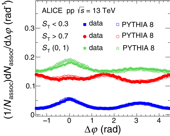
FIG. 2. The pion raw experimental distribution of the azimuthal angle difference \Delta\phi between the trigger and the associated particles for S_T > 0.7 (red circles), S_T < 0.3 (blue squares), and S_T(0, 1) (green stars) compared with MC PYTHIA 8 calculations shown with the corresponding open markers. The calculations include particle transport through the ALICE detector using the GEANT 3 transport package. The statistical uncertainties are smaller than the marker size.
