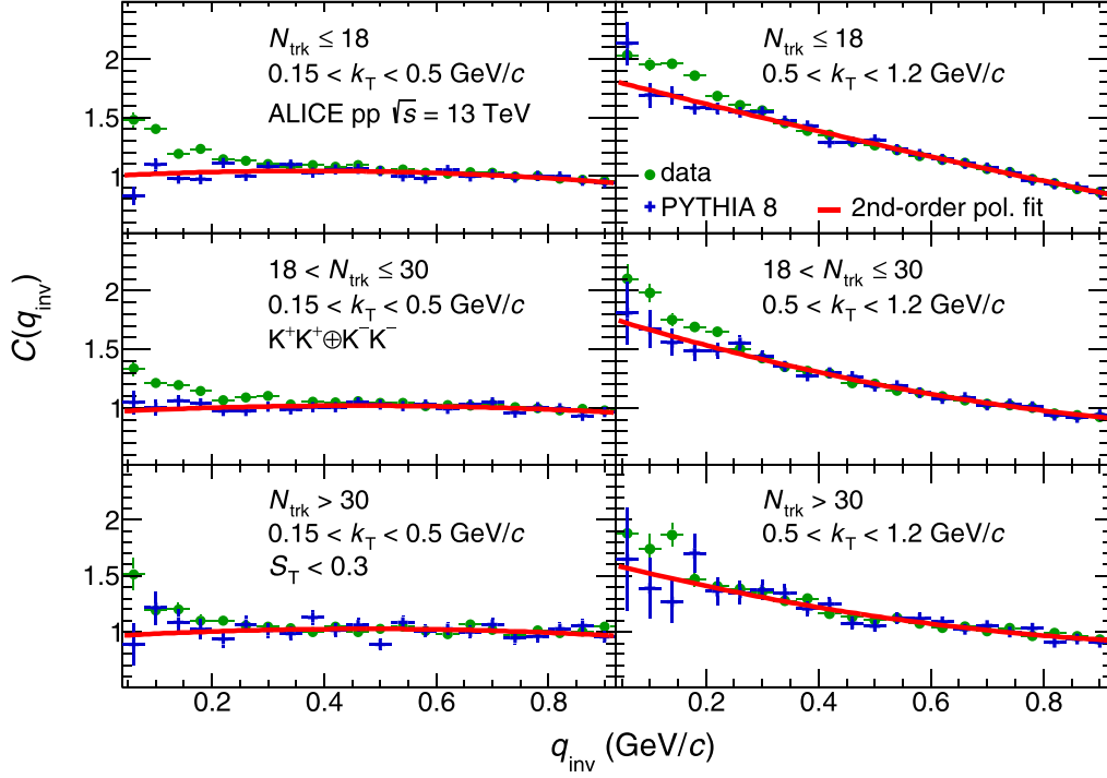
FIG. 6. The K^{\pm}K^{\pm} experimental correlation functions (green solid circles) as function of the invariant pair relative momentum q_{\text{inv}} in pp collisions at \sqrt{s} = 13 TeV for the raw multiplicity N_{\text{trk}} intervals of (1–18), (19–30), and ( >30 ) in the (0.15–0.5) and (0.5–1.2) GeV/ c k_T intervals. A sphericity selection of S_T < 0.3 is applied. The data are compared with PYTHIA 8 calculations, shown by blue crosses and approximated with a second-order polynomial (red curves). The error bars represent the statistical uncertainties, while the systematic uncertainties are negligible.
