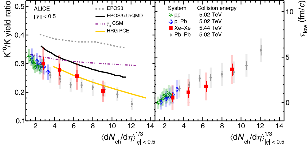
FIG. 5. The left panel shows the measured K^{*0}/K yield ratio along with model calculation. The right panel shows the lower limit of hadronic phase lifetime as a function of \langle dN_{\text{ch}}/d\eta \rangle_{|\eta| < 0.5}^{1/3} in different collision systems. Bars and shaded boxes represent the statistical and systematic uncertainties, respectively.
