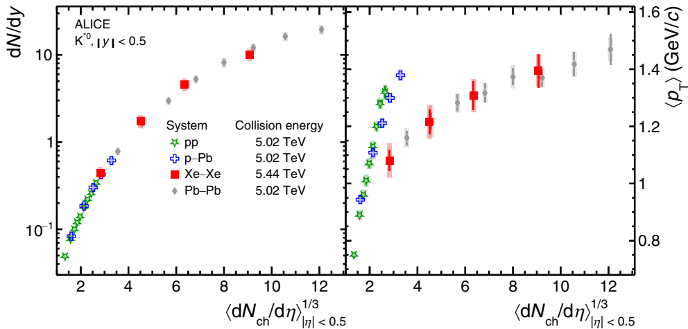
FIG. 4. The dN/dy (left panel) and \langle p_T \rangle (right panel) of K^{*0} as a function of \langle dN_{ch}/d\eta \rangle_{|\eta|<0.5}^{1/3} in pp collision at \sqrt{s} = 5.02 TeV and in Xe-Xe collisions at \sqrt{s_{NN}} = 5.44 TeV. Measurements are compared with the results obtained in p -Pb [5] and Pb-Pb [6] collisions at \sqrt{s_{NN}} = 5.02 TeV. Bars and shaded boxes correspond to the statistical and systematic uncertainties, respectively.
