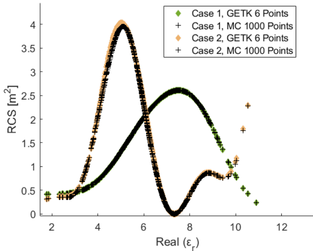
FIGURE 3. Comparison of output RCS surrogate reconstructions obtained by the novel GETK method, at 6 reconstruction points, with the reference 1000-point Monte Carlo (MC) simulations for the dielectric spherical scatterer analyzed in Fig. 1 (case 1) and that from Fig. 2 (case 2).
