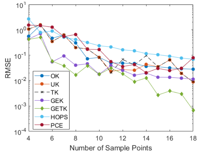
FIGURE 2. RCS reconstruction RMSE convergence for the five Kriging methods, HOPS, and PCE for a 2-m diameter spherical dielectric scatterer with input uncertain relative permittivity given by \epsilon_r = \{\sim N(6, 1.5), -1\} at 115 MHz. taking the reference 1000-point Monte Carlo results as an “exact” solution.
