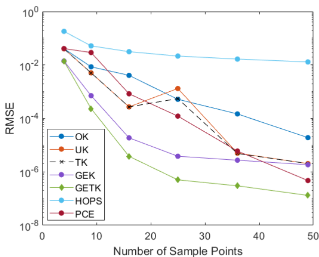
FIGURE 6. Convergence of the RMSE of the probability density function reconstruction versus the number of sample points using the five Kriging methods, HOPS, and PCE for the dielectric spherical scatterer with 2-D uncertainty analyzed in Fig. 5, with the 1000-point Monte Carlo simulation as a validation norm.
