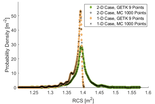
FIGURE 7. Comparison of the probability density reconstruction as a function of RCS QoI for the dielectric spherical scatterer with the 2-D parameter space from Fig. 5 generated by the novel GETK method at 9 reconstruction points with the reference 1000-point Monte Carlo solution. Overlaid are also the results for the 1-D random case in which the probability density of the imaginary part of \epsilon_r collapsed to its mean, \epsilon_r = \{N(4.5, 0.25), -1\} .
