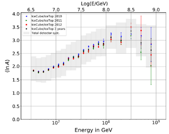
Fig. 8. Mean logarithmic mass \langle \ln A \rangle derived from the best fit to the neural network mass output for the 3 years of data and the individual years (Aartsen et al., 2019). The gray band represents the combined systematic uncertainties of the IceTop and in-ice detectors for the coincident analysis. Sibyll 2.1 was used for the hadronic interaction model.
