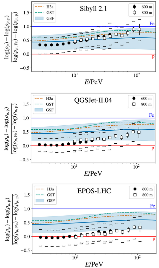
Fig. 12. Distribution of z -values as a function of the primary energy compared to various predictions from hadronic interaction models (Abbasi et al., 2022). Different flux model predictions are shown as lines. Error bars indicate statistical uncertainties, while brackets indicate systematic uncertainties. The blue band represents uncertainties obtained from the GSF flux model.
