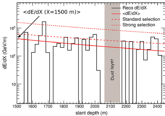
Fig. 5. An example of a reconstructed in-ice energy loss profile from a large event (Aartsen et al., 2019). The solid red line indicates the average energy loss fit, the dashed red line presents the standard stochastics selection, and the dotted red line is the strong stochastics selection. The gray band shows the approximate location of the dust layer.
