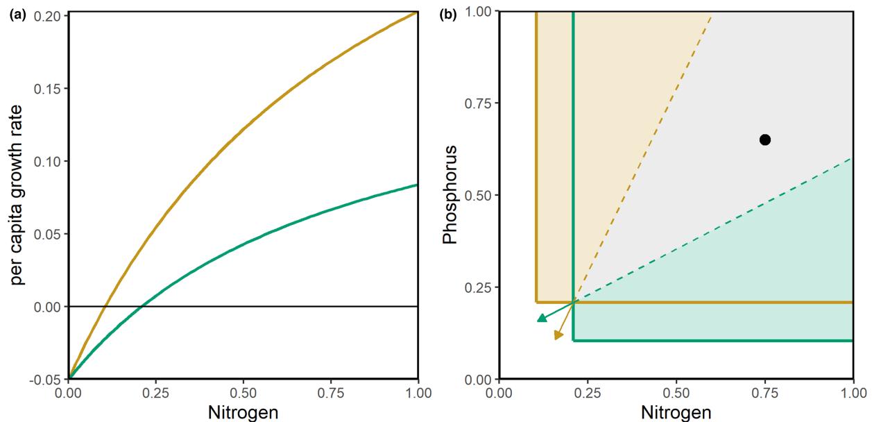
FIGURE 2 (a) State-space diagram of two hypothetical plant species (colored as green and gold) competing for one resource. The colored lines represent a species' per capita growth rate under different resource level. (b) State-space diagram of two hypothetical plant species competing for two essential resources. Here, we depict the coexistence criteria in terms of the elements of niche theory, i.e., the resource requirements (solid lines), the resource consumptions (solid arrows as consumption vectors), and the resource supply (black point). See box text for more details.
