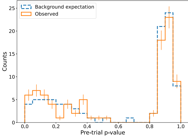
Figure 3. Pretrial p -value distribution of the 90 GW events followed up in this analysis (orange solid). This is compared to the background expectation of p -values (blue dashed). The observed p -value distribution is consistent with the background expectation.
