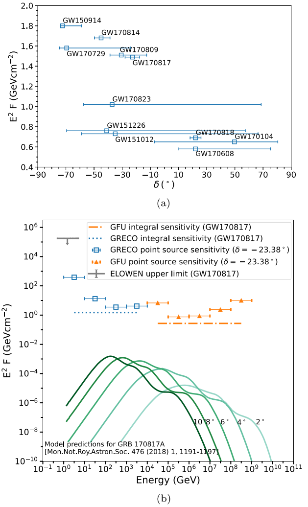
Figure 1. (a) Sensitivities of the GRECO Astronomy data set to the 11 GW events in the GWTC-1 catalog. The x-axis represents the decl. of the corresponding GW events (decl. with maximum probability shown by the squares and the decl. covering the 68% probability region shown as error bars). F represents the time-integrated flux as defined in Equation (3). The sensitivities for events in the Northern and Southern Hemispheres are within an order of magnitude. (b) The differential sensitivities of the GRECO Astronomy data set (in blue squares) compared to the differential sensitivities of the high-energy data set (GFU). The differential sensitivity curves are constructed by dividing the entire energy range into decadal bins. The GRECO Astronomy data set contains neutrinos of all flavors while GFU contains only muon neutrinos. Also shown are the integral sensitivities to a decl. corresponding to that of the host galaxy of GW170817, NGC 4993 (Coulter et al. 2017). The gray marker shows the flux upper limit on GW170817 obtained with the follow-up analysis using extremely low-energy neutrinos detected with IceCube (Abbasi et al. 2021). The green curves represent model predictions showing low-energy neutrino emission from a GRB like 170817A (Biehl et al. 2018). All sensitivities shown in (a) and (b) assume a spectral index of two for the flux.
