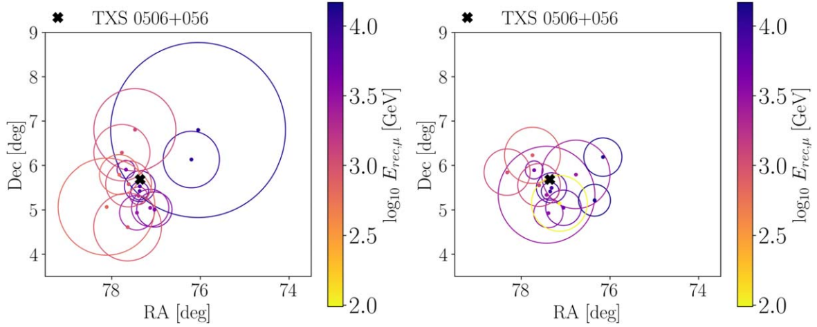
Figure 7. Position and energy (color) of the 14 events contributing the most to the TXS 0506+056 neutrino flare. The circles show the uncertainty of the directional reconstruction, \sigma_i . Left: the 14 most contributing events from the data sample used in this work (see Table 2). Right: the 14 most contributing events from the old data sample (Abbasi et al. 2021b).
