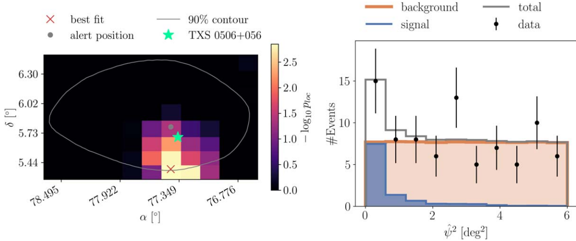
Figure 5. Left: p -value map of the alert region of IceCube-170922A. The gray dot indicates the reconstructed direction of IceCube-170922A, and the gray contour shows the 90% uncertainties of the reconstruction. The red cross marks the best-fit position of the position scan ( 0.6^\circ from the reconstructed alert position). The star shows the location of TXS 0506+056. All black bins have p -values close to 1. Right: number of events at binned squared angular distances, \hat{\psi}^2 , between TXS 0506+056 and the reconstructed event directions during the neutrino flare ( 57001 \text{ MJD} \pm 2 \times 64 days). Scrambled data in R.A. provide the background (blue), and Monte Carlo simulations for the best-fit flux ( n_S = 12 and \gamma = 2.31 ) yield the signal (orange). The gray line combines the background with the signal and matches the data points (black). The data are shown with 68% uncertainties.
