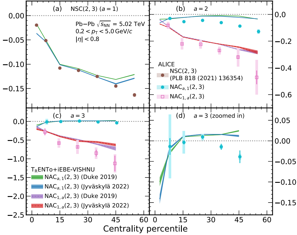
FIG. 2. Centrality dependence of the different orders a = 1, \dots, 3 of \text{NAC}_{a,1}(2, 3) (cyan closed circles) and \text{NAC}_{1,a}(2, 3) (pink open squares) compared with the theoretical predictions from \text{T}_\text{R} \text{ENTo} + \text{iEBE-VISHNU} for the Duke 2019 [22] and Jyväskylä 2022 [12] parametrizations. Panel (d) shows a close-up of the results of \text{NAC}_{3,1}(2, 3) . The statistical uncertainties in the calculations are indicated by the thicknesses of the colored bands. The data points for \text{NSC}(2, 3) are taken from Ref. [17].
