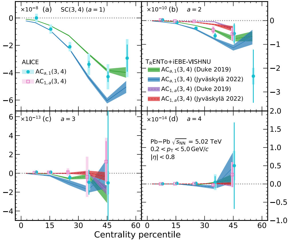
FIG. 9. Centrality dependence of the different orders a = 1, \dots, 4 of AC_{a,1}(3, 4) (cyan closed circles) and AC_{1,a}(3, 4) (pink open squares) compared with the theoretical predictions from T_{\text{REnto}} + \text{iEBE-VISHNU} for the Duke 2019 [22] and Jyvaskylä 2022 [12] parametrizations. The statistical uncertainties in the calculations are indicated by the thicknesses of the colored bands.
