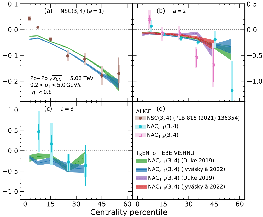
FIG. 4. Centrality dependence of the different orders a = 1, \dots, 3 of \text{NAC}_{a,1}(3,4) (cyan closed circles) and \text{NAC}_{1,a}(3,4) (pink open squares) compared with the theoretical predictions from \text{T}_\text{R} \text{ENTo} + \text{iEBE-VISHNU} for the Duke 2019 [22] and Jyväskylä 2022 [12] parametrizations. The statistical uncertainties in the calculations are indicated by the thicknesses of the colored bands. The data points for \text{NSC}(3,4) are taken from Ref. [17].
