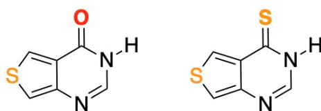
Scheme 1. Molecular structures of ThiaHX (left) and ThiathioHX (right). Note, while this heterocyclic system is numbered differently than the native purines, we will use the latter nomenclature for familiarity and clarity throughout this study. Thus, we will consider the carbonyl and thiocarbonyl positions as C6. See ESI for synthesis, characterization data, and crystal structures.
