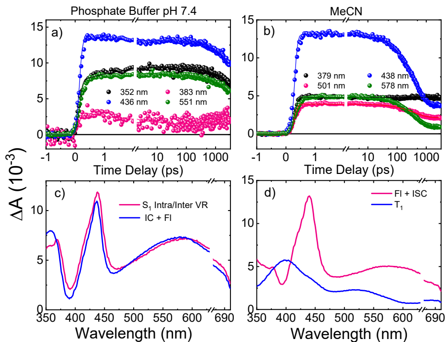
Figure 4. Representative decay traces of ThiaHX in a) phosphate buffer and in b) MeCN upon excitation with 325 nm. Evolution-associated difference spectra (EADS) of ThiaHX in c) phosphate buffer and in d) MeCN, extracted from the global and target analyses. VR, FI, IC and ISC stand for vibrational redistribution, fluorescence, internal conversion, and intersystem crossing, respectively. The breaks are covering the overtone of the pump beam at 650 nm.
