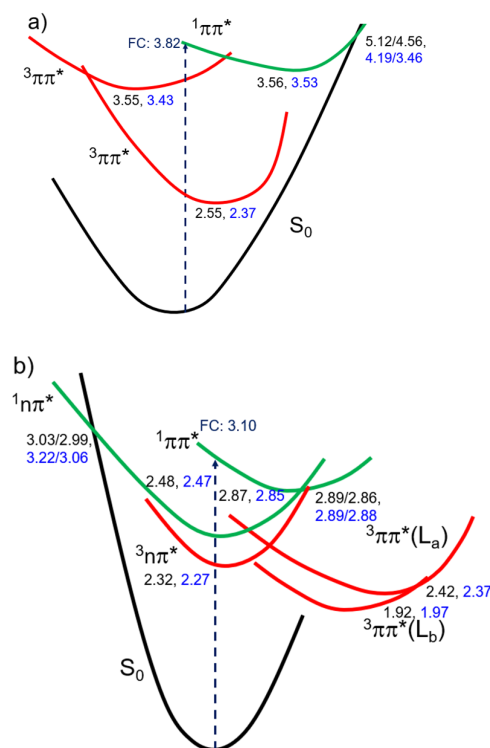
Figure 3. Proposed order of the four lower energy electronic states for ThiaHX (a) and the five lower energy states of ThiathioHX (b) in MeCN (values shown in black) and water (values shown in blue) based on the calculations reported in this work. Values correspond to relative energies (in eV) of key stationary points, conical intersections, and crossing points.
