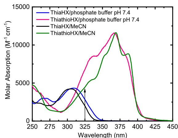
Figure 1. Absorption spectra of ThiaHX and ThiathioHX in phosphate buffer (pH 7.4) and MeCN. The vertical arrow shows the excitation wavelength used in the femtosecond transient absorption experiments of 325 nm.
