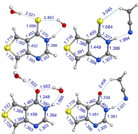
Figure 2. Ground-state optimized structures of ThiathioHX in water (top, left) and MeCN (top, right) and ThiaHX in water (bottom, left) and in MeCN (bottom, right) obtained at the CASPT2/cc-pVDZ level of theory.
