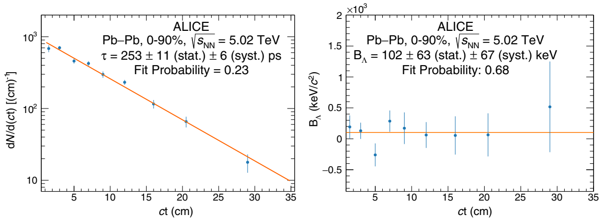
FIG. 1. Left: exponential decay spectrum as a function of the proper decay length for {}^3_\Lambda\text{H} , the blue points represent the measured yield, while the orange line represents the best fit to the measurement. Right: B_\Lambda measurement as a function of the proper decay length. Only statistical uncertainties are shown; see the text for a description of the determination of the systematic uncertainties. The fit probability computed with a Pearson test is reported.
