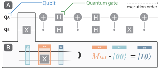
Fig. 1. (A) An example quantum circuit reproduced from the prior work [22], which consists of qubits and quantum gates. (B) The intuitive illustration that shows how the matrix multiplication is performed given the quantum gate and initial quantum state.
