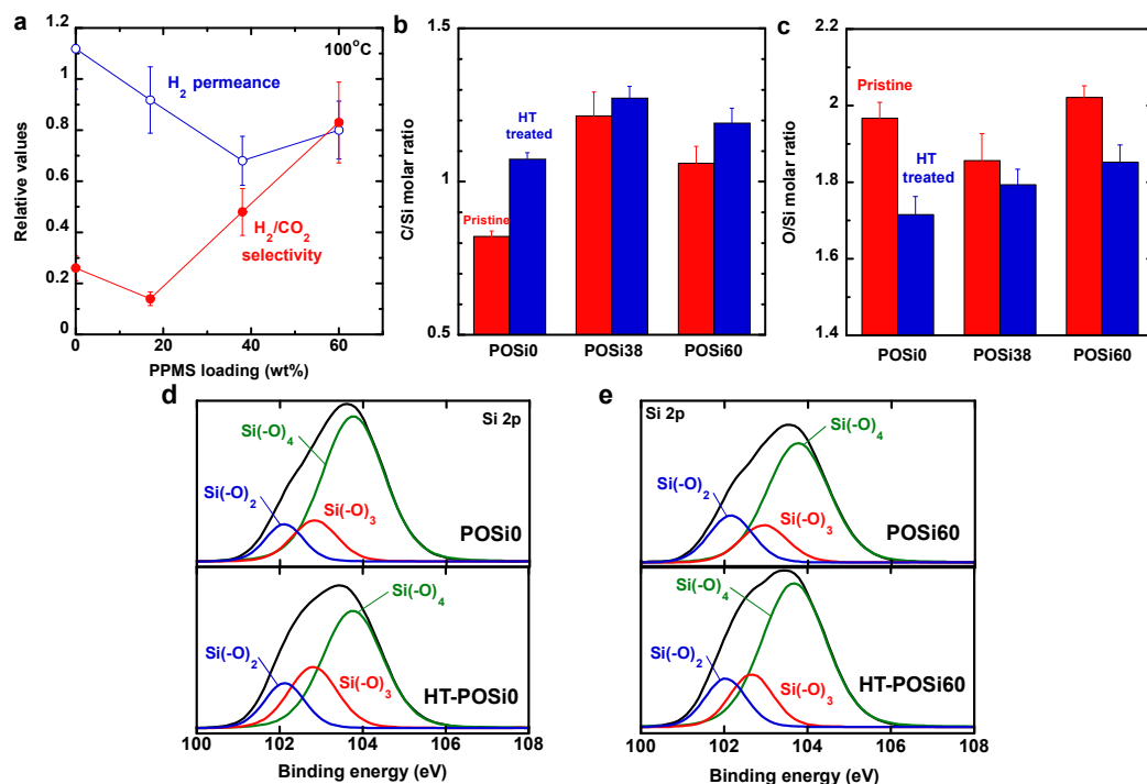
Fig. 5 Hydrothermal stability of POSi membranes after exposure to saturated water vapor at 100 °C for 12 h. (a) Relative H 2 permeance and H 2 /CO 2 selectivity. (b) C/Si molar ratio and (c) O/Si molar ratio. Si 2p peak deconvolution of (d) POSi0 and (e) POSi60.
