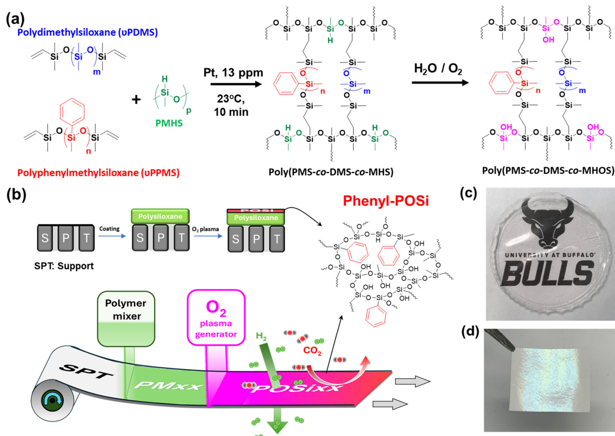
Fig. 1 Our approach of POSi membranes (POSixx) derived from poly(PMS-co-DMS-co-MHOS). (a) Synthesis of poly(PMS-co-DMS-co-MHOS) by hydrosilylation reaction followed by hydrolysis and oxidation of the unreacted Si-H groups. (b) Preparation of POSi membranes, including fabrication of polysiloxane TFC membranes (PMxx) and oxygen plasma treatment. Photos of (c) a freestanding polysiloxane film and (d) a POSi membrane.
