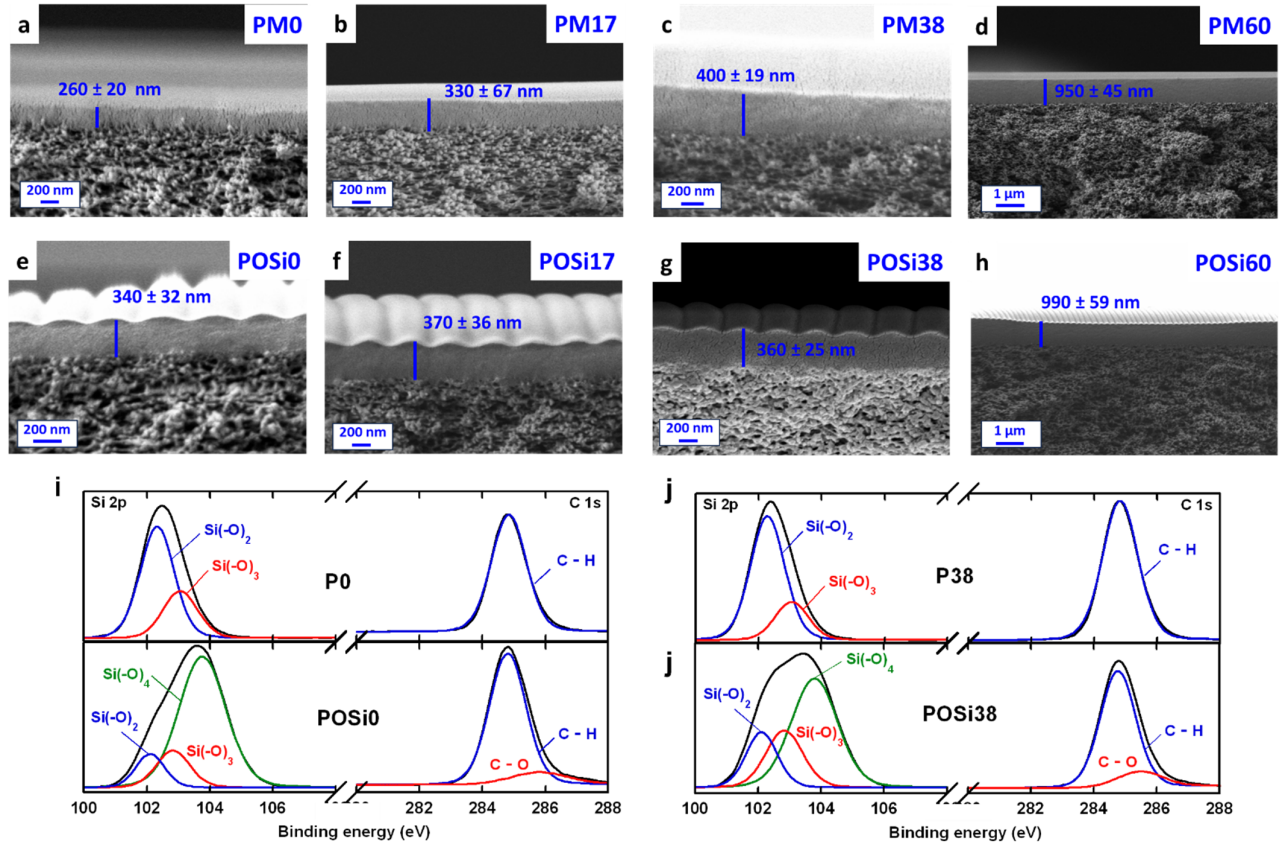
Fig. 3 Cross-sectional SEM images for the membranes of (a) PM0, (b) PM17, (c) PM38, (d) PM60, (e) POSi0, (f) POSi17, (g) POSi38, and (h) POSi60. Comparison of Si2p and C1s peaks (i) between P0 and POSi0 and (j) between P38 and POSi38 by XPS.
