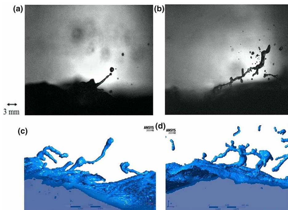
Figure 2. Formation of spray droplets in a laboratory apparatus (a,b) and in direct numerical simulations (c,d), under tropical cyclone-like conditions (10-m wind speed of 40 \text{ ms}^{-1} ). Panels (a) and (c) pertain to a pure water surface, whereas a surfactant has been added in (b) and (d). From [25].
