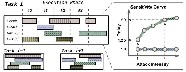
Fig. 4: Profiling resource contention sensitivity for tasks.
