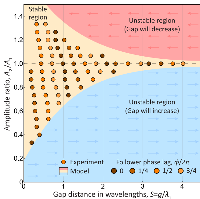
Fig. 3. Stable positions for the follower for varying amplitude ratio A_2/A_1 and phase difference \phi at equal frequency in experiment (circles) and model (background color). At fixed \phi , increasing A_2/A_1 compresses the pair, while decreasing A_2/A_1 leads to an increase in S , up to some threshold.
