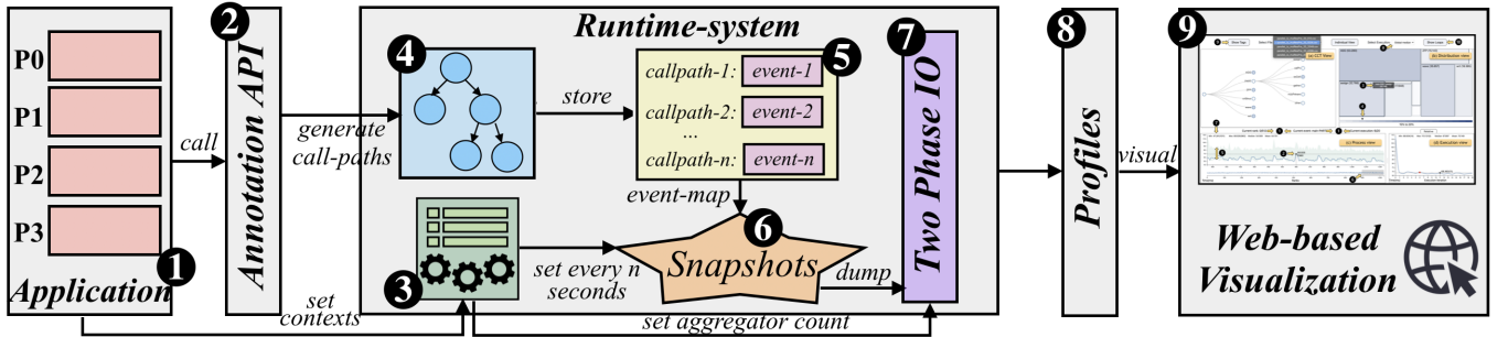
Fig. 1: The workflow of TinyProf . An application begins by setting one-time, global application-specific contexts (③). Then the annotation API (②) invokes a series of profiled code regions (events). The runtime is responsible for generating the unique key called as callpath of every event (④) which then gets stored in an event-map (⑤). TinyProf provides the ability to snapshot (⑥) the entire state of performance metric every n seconds, an important fault tolerant measure. To reduce the file I/O overhead, we have developed a three-phase I/O technique (⑦) to dump performance metrics in a customized compact file format (⑧). The profiles can then be read by most existing visualization tools (⑨).
