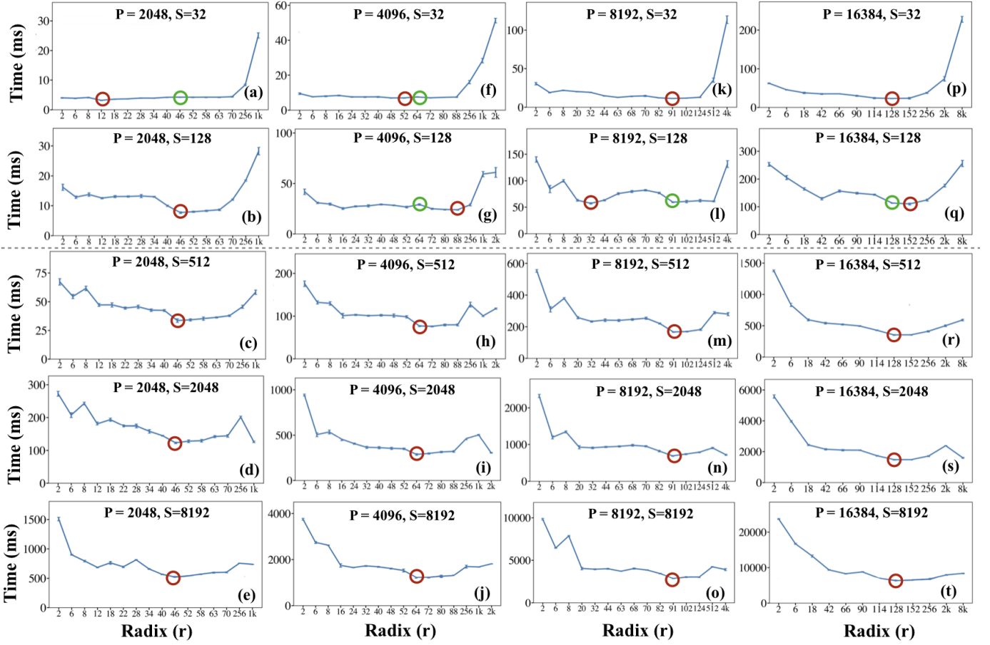
Fig. 8: Performance analysis of TRA on Theta with varying process count ( P ), size per data-block ( S ), and radix ( r ). A red circle highlights the best r with optimal performance in each figure, while a green circle indicates r = \sqrt{P} when it is not equal to the best radix. ( \lceil \sqrt{2048} \rceil = 46 , \sqrt{4096} = 64 , \lceil \sqrt{8192} \rceil = 91 , \sqrt{16384} = 128 ).
