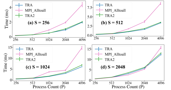
Fig. 12: Performance comparison of TRA with optimal radix ( r = \sqrt{P} ), TRA2 with optimal radices ( r_1 = \sqrt{Q} (intra), r_2 = N (inter)), and MPI_Alltoall on Polaris.
