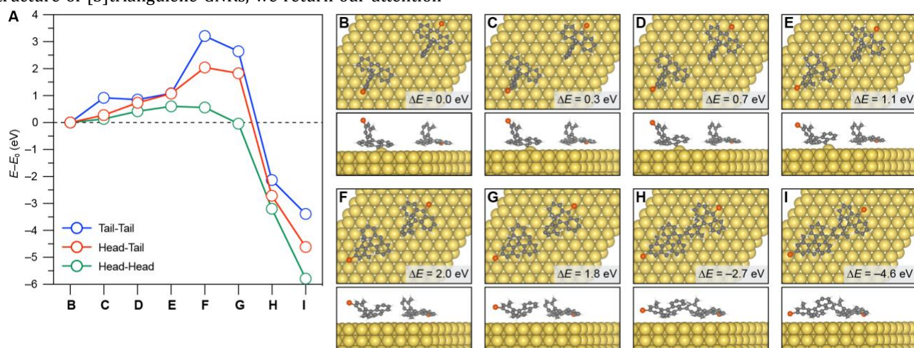
Figure 4. Mechanistic calculations of the regioselective coupling of molecular precursor 1 on Au(111). (A) Calculated reaction coordinate diagram showing transition state energies corresponding to the head-to-tail (HT), head-to-head (HH), and tail-to-tail (TT) coupling geometries. (B) Minimized geometries of molecular precursor 1 , (C–H) intermediates, and (I) the product dimer along the head-to-tail coupling pathway.
