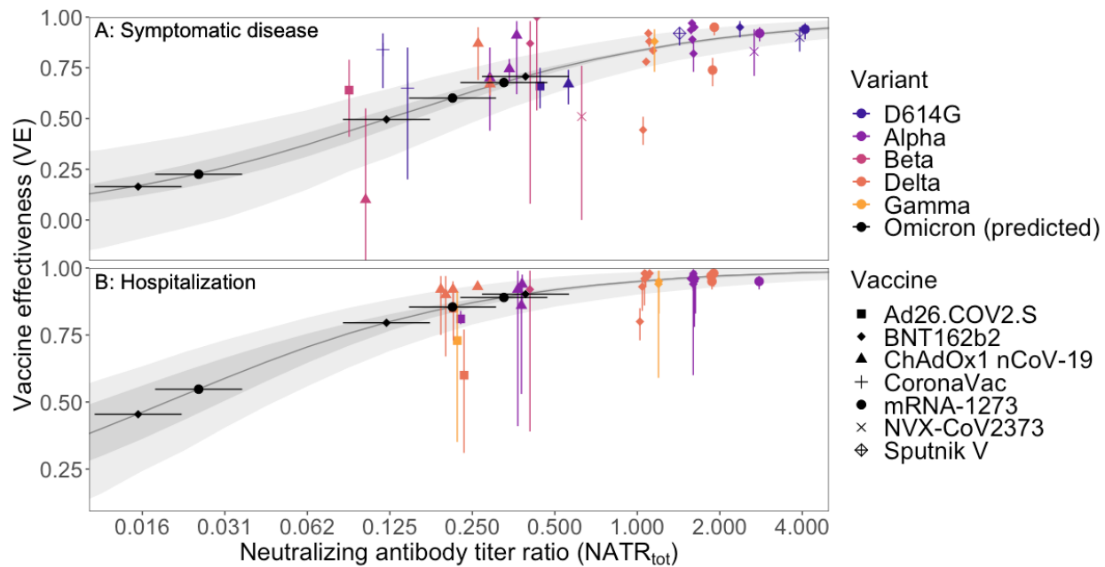
Figure 2. Vaccine effectiveness (VE) plotted against variant- and vaccine-specific neutralizing antibody titer ratios (NATR tot ) for (A) symptomatic disease and (B) hospitalization. Each point (and 95% CI), except those for Omicron predictions, represents a single empirical estimate of VE for a single vaccine and virus variant (Tables S4 and S5). Points are jittered slightly along the x-axis to facilitate presentation. Black points show predicted values for the Omicron variant using the fitted model (Table S6); horizontal error bars show 95% CIs for Omicron-specific neutralizing antibody titer ratios from Figure 1. Dark ribbons show 95% CIs for the fitted model, and lighter ribbons show 95% prediction intervals with a mean of 115 infections in the unvaccinated control group (see Section 2).
