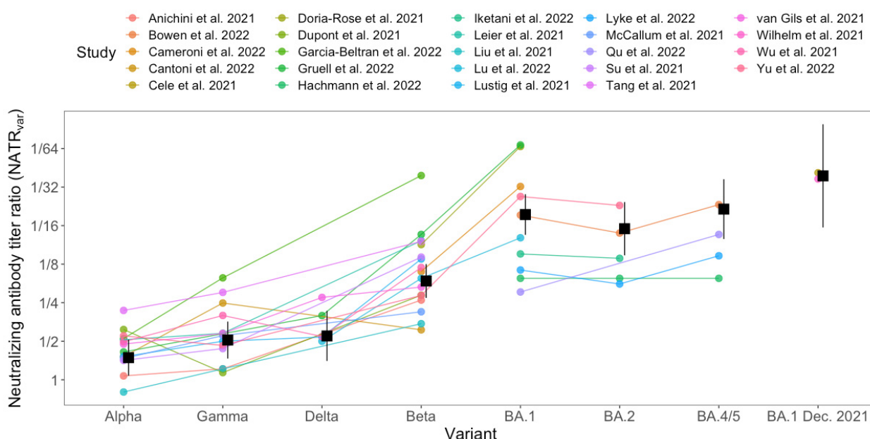
Figure 1. Neutralizing antibody titer ratios for virus variants relative to WT virus ( NATR_{var} ) for five SARS-CoV-2 variants and three subvariants. Each point shows the reduction in neutralizing antibody titer relative to WT virus for a specific vaccine against a virus variant (Table S1). Colors and lines connect points from the same study. Black squares and error bars show the mean and 95% confidence interval for each variant from the fitted model.
