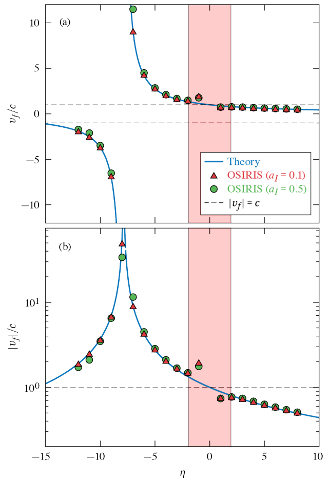
FIG. 4. Comparison of the focal velocities predicted by the “thick” lens theory [Eq. (24)] and the PIC simulations as a function of the chirp parameter \eta . The theory and simulations are in excellent agreement when the effective duration \tau_f is larger than the stretched pulse duration (outside the red shaded area).
