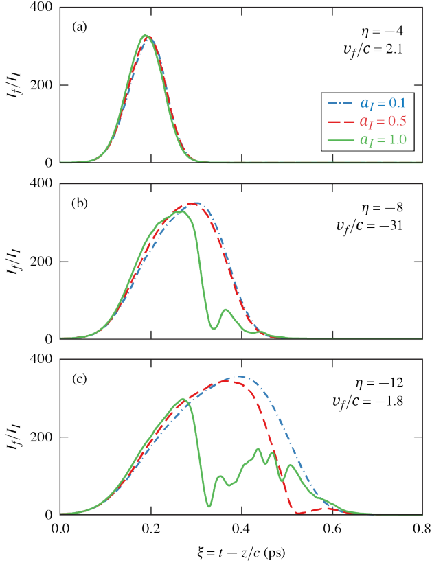
FIG. 5. Temporal profiles of the on-axis intensity at the nominal focal point z = L_p + f_l(\omega_0) for three different focal velocities (or chirps \eta ) and incident amplitudes a_I . In all cases, the intensity is normalized to the incident intensity I_I . Pulses with longer durations and larger amplitudes are more susceptible to modifications due to nonlinear propagation and plasma evolution.
