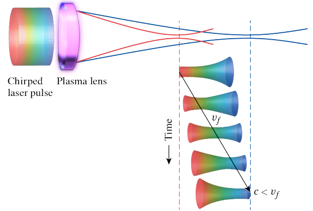
FIG. 1. A chirped laser pulse focused by a plasma lens results in a moving, or “flying,” focus with an intensity peak that moves independently of the group velocity. The plasma lens focuses different frequencies to different longitudinal locations, while the chirp controls the arrival time of the frequencies at these locations. In this case, the velocity of the moving focus is superluminal ( v_f > c ).
