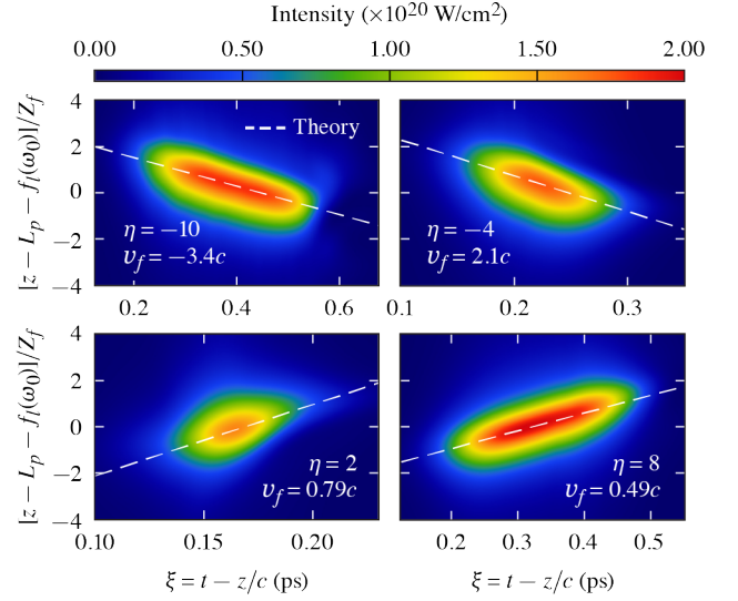
FIG. 3. Spatiotemporal profiles of the moving focus within the focal range for different focal velocities v_f (or chirps \eta ) at r = 0 . The intensity peak has a near-constant velocity and a maximum intensity that is consistent with the theory. In each case, the incident laser pulse had a normalized amplitude a_I = 0.5 . The distance from the nominal focus f_I(\omega_0) is normalized to the Rayleigh range of the focused spot at the central frequency Z_f \equiv c w_f^2/2\omega_0 .
