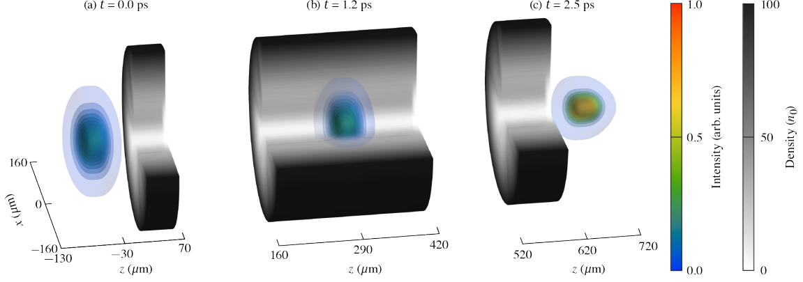
FIG. 2. Density contours of the plasma lens (grey scale) and intensity contours (color scale) of a laser pulse traversing the plasma lens. For this design, the plasma lens is “thick,” and the spot size of the laser pulse decreases appreciably from the entrance to the exit of the lens (left to right). The incident laser pulse has a normalized amplitude a_I = 0.5 and chirp parameter \eta = -5 . All other parameters can be found in Table I.
