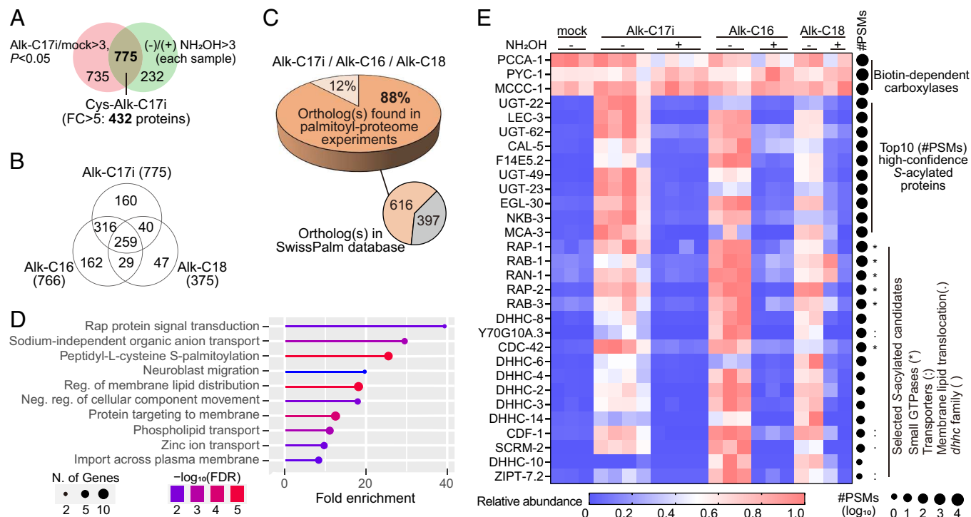
Fig. 4. Profiling of protein S-fatty acylation in C. elegans . (A) Overlap of Alk-C17i-enriched and hydroxylamine-cleavable proteins are cysteine isoC17:0-modified candidate proteins. FC, fold-change in both filters. (B) Number of S-acylated protein candidates identified using the three probes. Alk-C17i, n = 4 ; Alk-C16, n = 3 ; Alk-C18, n = 2 . (C) Comparison of identified C. elegans S-acylated proteins with existing S-acylation data in the SwissPalm database. 616 of the 1,013 S-acylated C. elegans proteins have annotated orthologs in at least one of the species used in the SwissPalm-documented S-acyl-proteome experiments (91 experiments with 12 organisms; no experiments with C. elegans have been published). Orthologs of 88% of these 616 C. elegans proteins have been found in previous S-acyl-proteome experiments. (D) Biological process gene ontology analysis for C. elegans S-acylated proteins (Alk/mock > 5 and (-)/(+) \text{NH}_2\text{OH} > 5 in least one probe group). (E) Heat map of abundances of selected proteins including biotin-dependent carboxylases and S-acylated candidates. #PSMs, number of peptide spectrum matches in all samples.
