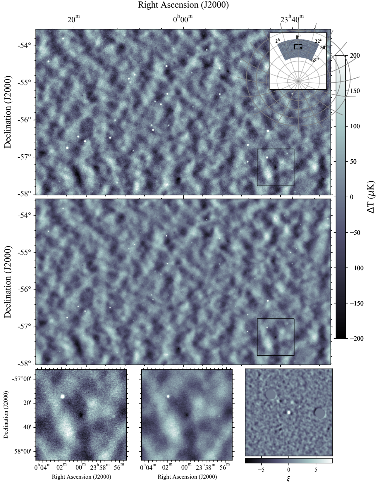
Figure 1. Sequentially zoomed-in images of the SPTpol 500d field, with the full field shown in inset at top. (Top panel) 24 deg 2 of 95 GHz data (Middle panel) The same region at 150 GHz. The full field temperature maps and associated data products are released along with this work. (Bottom panel) To better illustrate the sensitivity of these maps to small scales, we further zoom in to a 1.25 × 1.25 degree region (outlined in black in above panels) centered on SPT-CL J2341-5724, a \xi = 14.3 cluster at z = 1.259 . Plotted from left-to-right are the 95 and 150 GHz temperature maps and the \xi -map constructed for optimal detection of clusters with \theta_{\text{core}} = 0.25 . Sources brighter than 6 mJy at 150 GHz were masked in the cluster detection step, with two examples visible in the bottom right panel.
