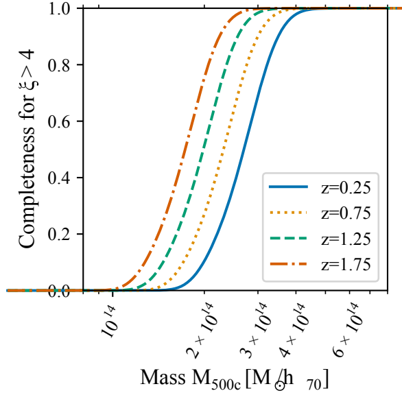
Figure 11. Expected completeness of the \xi > 4 SPTpol sample as a function of M_{500c} at several redshifts. The sample is expected to be > 90\% complete at M_{500c} > 3.5 \times 10^{14} M_{\odot}/h_{70} at z > 0.25 . At lower redshifts the atmospheric filtering removes larger angular-scale cluster signals leading the sample to be increasingly incomplete at z < 0.25 .
