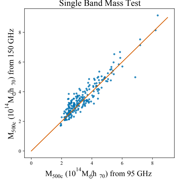
Figure 8. Masses estimated from 95 and 150 GHz data alone for 250 clusters individually detected in each band. Overall we find excellent agreement between the two, with the largest outlier, SPT-CL J2332-5358 ( 5.4\sigma , at a ratio of M_{95\text{ GHz}}/M_{150\text{ GHz}} = 7/5 ) having previously been identified as a cluster-scale strong lens of a distant star forming galaxy whose emission results in significantly reduced tSZ signal in 150 GHz data.
