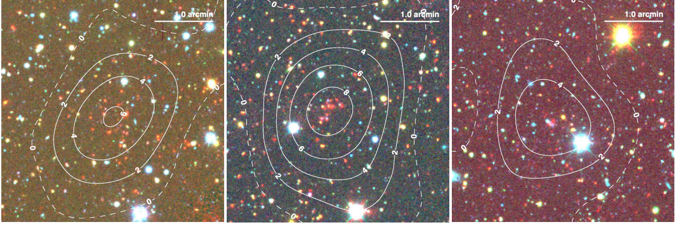
Figure 10. Three of the high- z clusters discovered in the SPTpol 500d survey. From left to right, SPT-CL J0128-5222 at \xi = 6 and z = 1.4 \pm 0.07 , SPT-CL J0122-5801 at \xi = 9 and z \geq 1.6 , and SPT-CL J0116-5039 at \xi = 6 and z \geq 1.6 . The SZ detection contours are overlaid on RGB images from Spitzer [3.6] and DES i - and g -band data. Star formation—as traced by bluer emission correlated with the galaxy overdensities—is prominently visible in some of these high- z cluster galaxies, highlighting the ability of this sample to probe clusters in the high- z transitional era between active star formation and passive galaxy evolution. SPT-CL J0122-5801 is one of the systems tagged as having multiple overdensities along the line-of-sight, with an additional foreground system of \lambda = 16 , z = 0.6 , and f_{\text{cont}} = 0.05 . The deep high-resolution Spitzer data allow us to detect the more significant distant background cluster.
