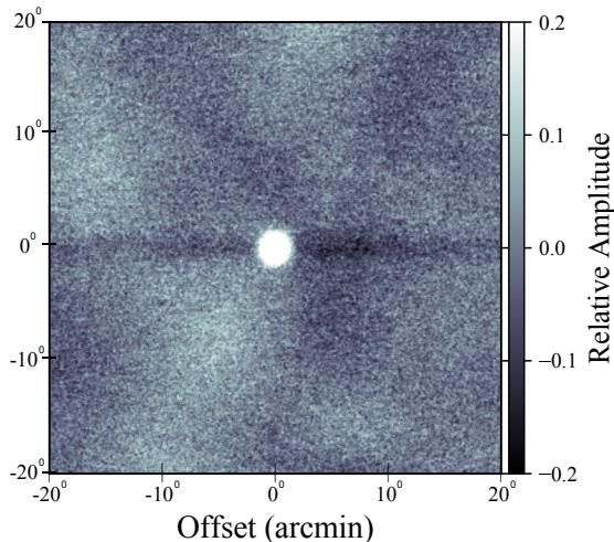
Figure 2. 40' \times 40' normalized median stack of sources at 95 GHz used to make the source subtraction template; a similar template was constructed at 150 GHz. The negative filtering artifacts along the scan (horizontal) direction are clearly visible even in these stacks which have significant residual large scale noise contributions from the primary CMB.
