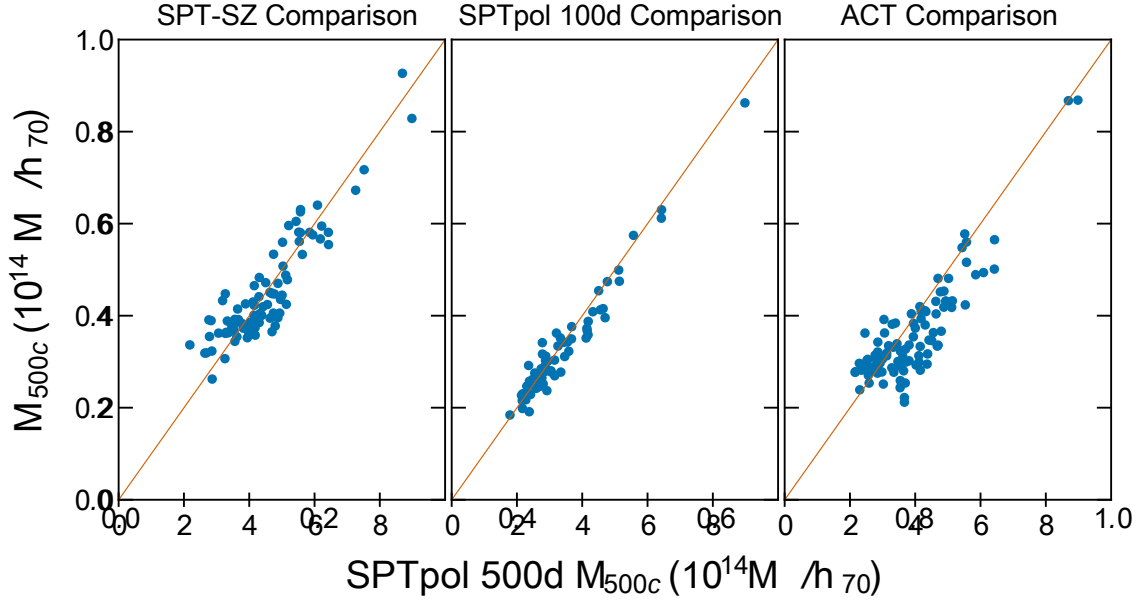
Figure 12. Comparisons of mass estimates for clusters from SPTpol 500d that are in common with systems in SPT-SZ (Bleem et al. 2015), SPTpol 100d (Huang et al. 2020), and ACT (Hilton et al. 2021). Over-plotted is a line representing a one-to-one relationship. As discussed in Section 8.1, we find good agreement between the 3 SPT surveys, with the median ratio of masses of SPTpol 500d/SPT-SZ to be 1.02^{+0.02}_{-0.04} and SPTpol 500d/SPTpol 100d to be 1.02 \pm 0.02 . We do note a small ( 2.3\sigma ) difference in the normalization of the ACT and SPT masses, finding the ratio of masses from SPTpol 500d/ACT = 1.07 \pm 0.03 (differing from the consistency shown in Hilton et al. 2021), but a stronger test of any cross experiment mass calibration differences will come when comparing weak-lensing calibrated samples in future works.
